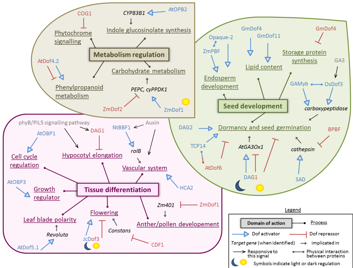
Figure I-5: Examples of some processes which are known to involve regulation by DOF transcription factors (the genes described are detailed in table II-3 and section I-2-9).
