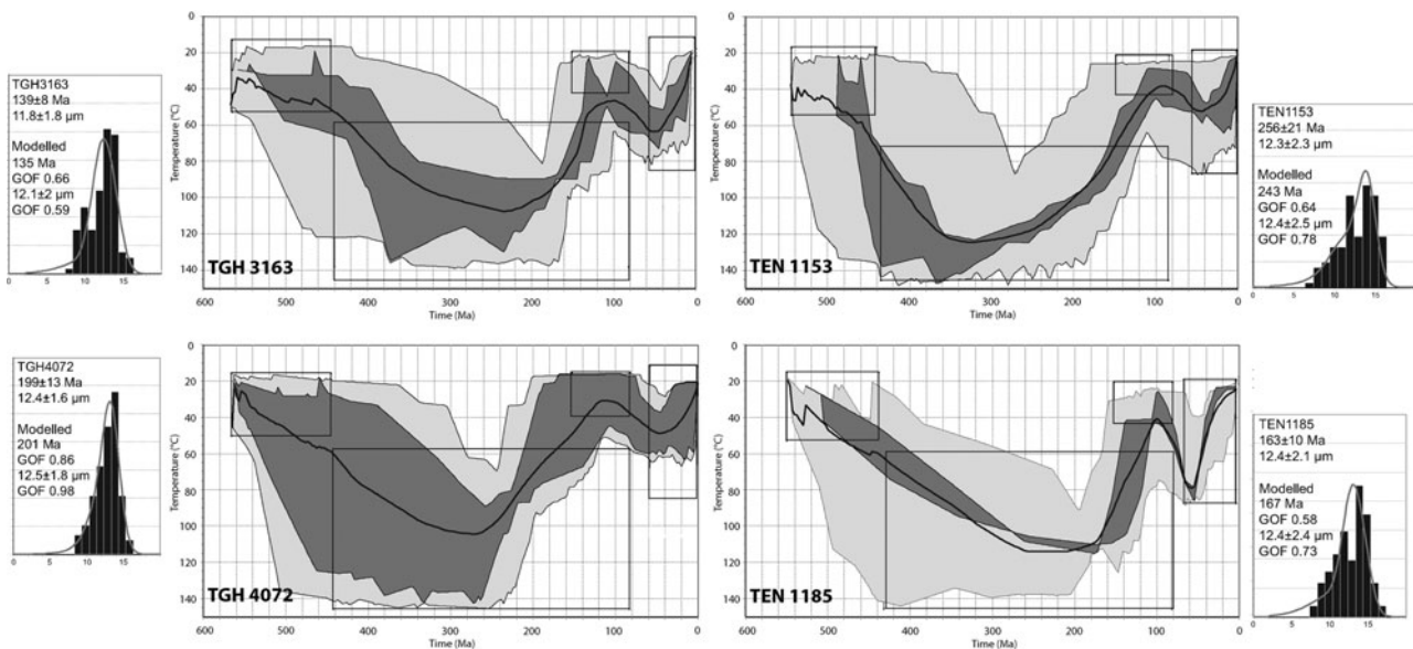
Figure 5. Thermal modelling for the model 2. Same legend as Figure 4.
