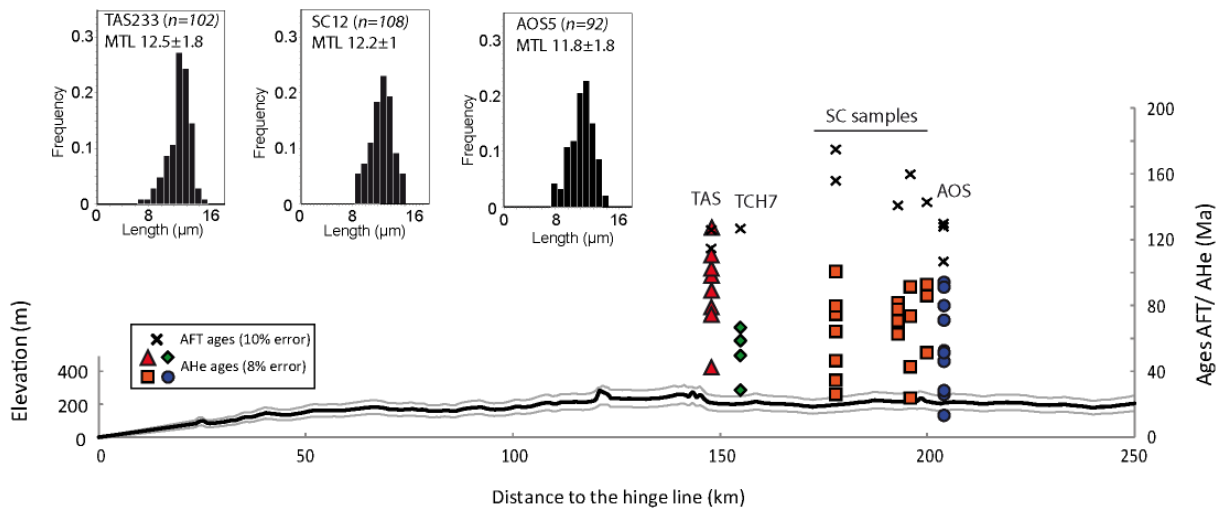
Figure IV-8 : Cross-section of the onshore margin (profile 1 on Figure IV-7a) with geographical distribution of the thermochronological data (AFT and corrected AHe ages). Same legend than in Figure IV-7 for each sample. The locations of the various sampling sites are projected along a section perpendicular to the coast. The fission tracks lengths data are given for three representative samples TAS233, SC12 and AOS5 given they provided sufficient lengths to measure. Other samples from SC and AOS groups show similar length distributions, whereas we did not use length distribution for TCH7 as it carried too few ( n = 37 ). Light grey lines show the maximum variation in elevation within 50 km from the main cross-section (black line).
