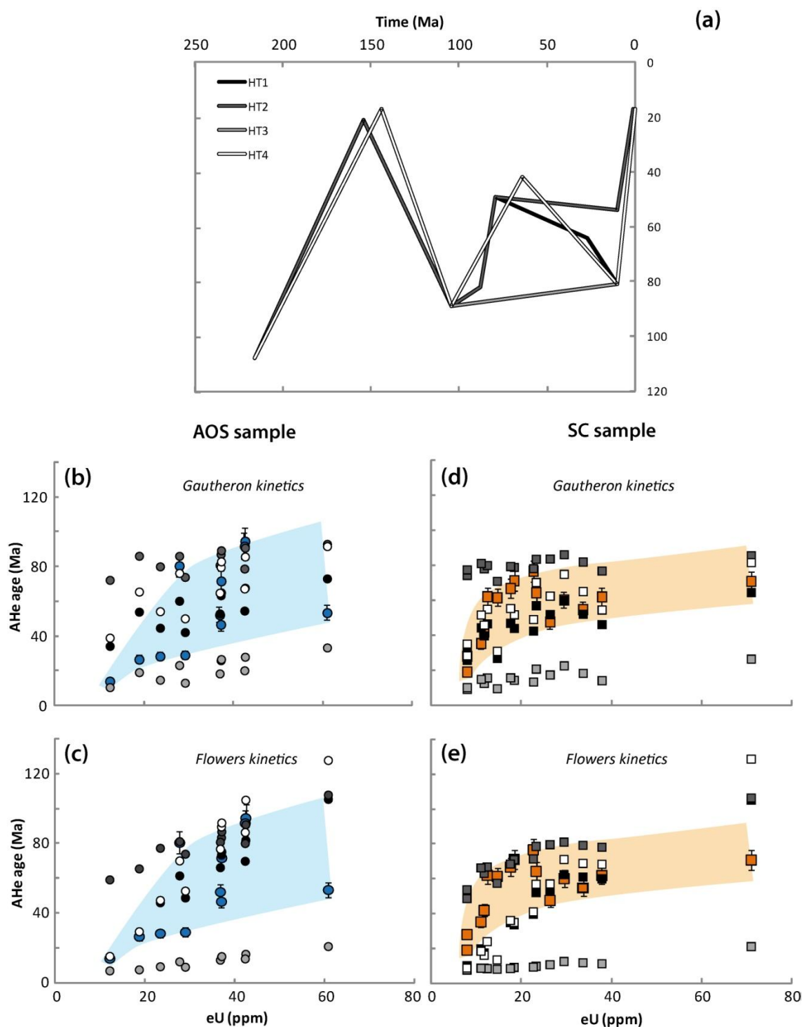
Figure S7. Forward modeling results. (a) Four different thermal paths are tested, HT1 (black), HT2 (dark grey), H3 (light grey) and HT4 (white). (b, c) AHe age-eU plots for AOS grouped sample. Blue circles show the measured data. Black, dark and light grey and white circles show the predicted data for the corresponding tested thermal paths. (d,e) AHe age-eU plots for SC grouped sample. Black, dark and light grey and white squares show the predicted data for the corresponding tested thermal paths. For each plot, the maximum dispersion of the measured data is underlined with a colored spindle (blue for AOS and orange for SC), allowing a better comparison with the predicted data (see Text S1).
