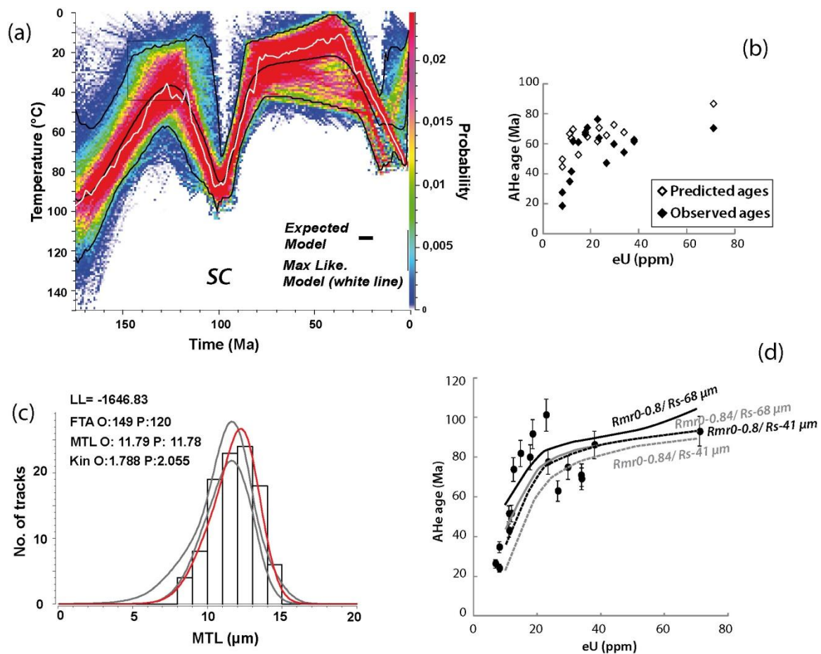
Figure S8. Alternative final modeling for SC sample, processed with the Flowers et al. [2009] code for the radiation damage and annealing. (a) Thermal history. Black box indicates the stratigraphical constraint of the Early Cretaceous. Max. Like: Maximum likelihood model. (b) Predicted AHe ages against observed AHe ages. (c) Predicted lengths distribution (grey and red curves), Mean Track Length (MTL) and Dpar (Kin) against the observed ones. FTA: Fission Track Age; O: Observed; P: Predicted; LL: Log Likelihood. (d) Predicted AHe-eU relationships for the thermal history of the expected model (black line in (a)) given the r_{mr0} and the grain size ranges.
