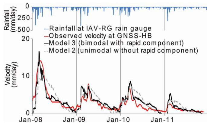
Figure 8.12 : The results for the HB landslide model. In blue, the daily rainfall at the IAV rain gauge; red line, the observed velocities at station GNSS-HB; black line, the results of the bimodal impulse model calibrated over period 2; dashed grey line, the results of the unimodal impulse model calibrated over period 2 (CP2).
