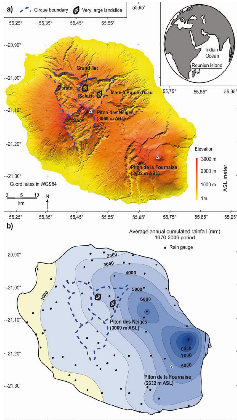
Figure 8.1 : a) Reunion Island DEM at a 25-metre resolution. In blue, the contours of the Mafate, Cilaos, and Salazie cirques. The landslide locations in the Salazie cirque. b) The rainfall spatial distribution on Reunion Island, simplified and modified from Météo-France datas (Météo-France, 2011).
