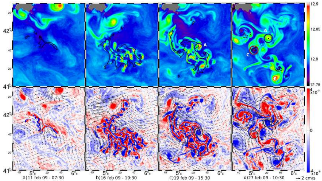
FIGURE E.2 – Temporal evolution at important stages of the formation of the eddies, with (top row) potential temperature at 1800 m depth and (bottom row) relative vorticity on isopycnal \sigma_0=1029.1 \text{ kg.m}^{-3} and (grey arrows) velocity field. In the top row, (black line) the 2000 m mixed layer depth contour is superimposed. Circles represent (red) the cyclone labelled C and (blue) the anticyclone labelled A, described in greater detail. The grey shaded area shows where the bottom is above 1800 m.
