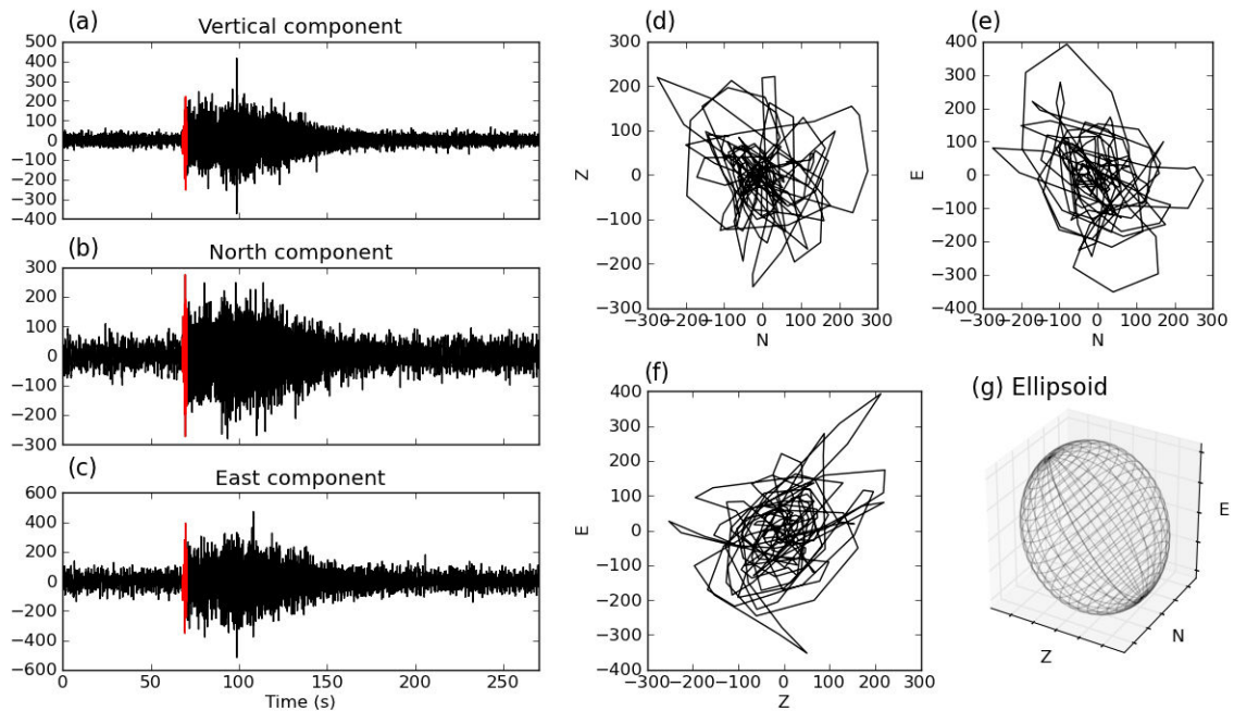
(b) EB
