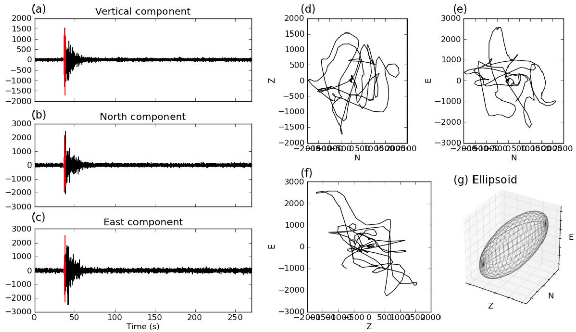
(a) VT
