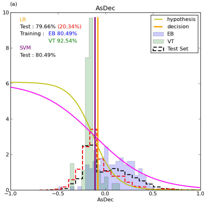
(a) AsDec
