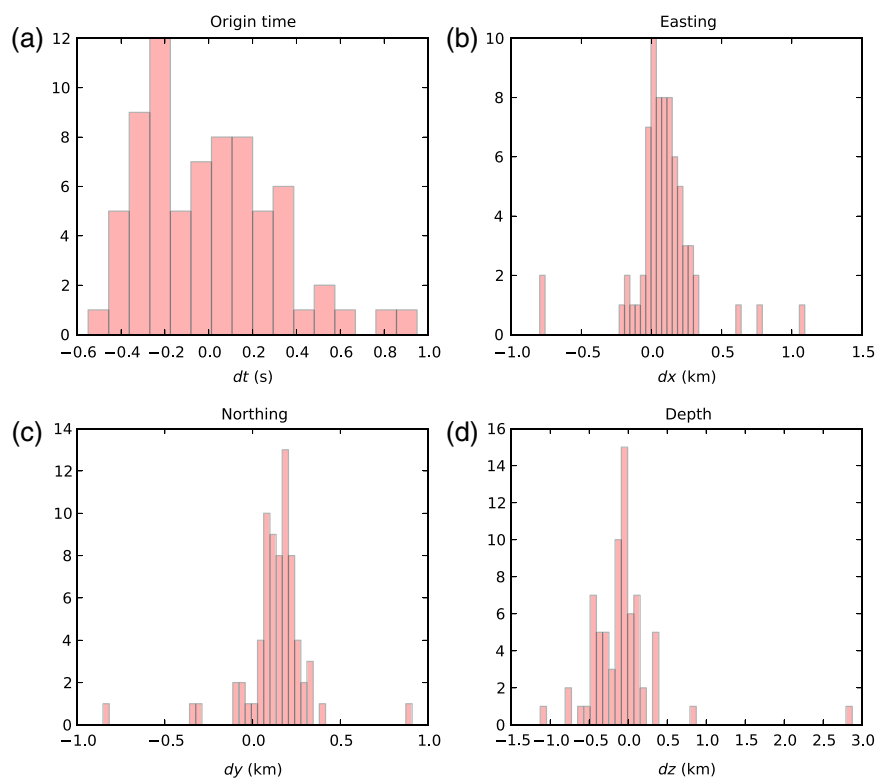
Figure 11. Comparison of Waveloc and the OVPF hypocentral parameters for the 72 locations provided by OVPF. The color version of this figure is available only in the electronic edition.
