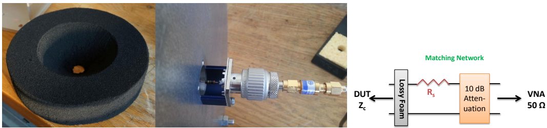
Figure 6.15: Matching Network for the "stretched wire" technique composed of attenuators, matching resistor and absorbing foam.
