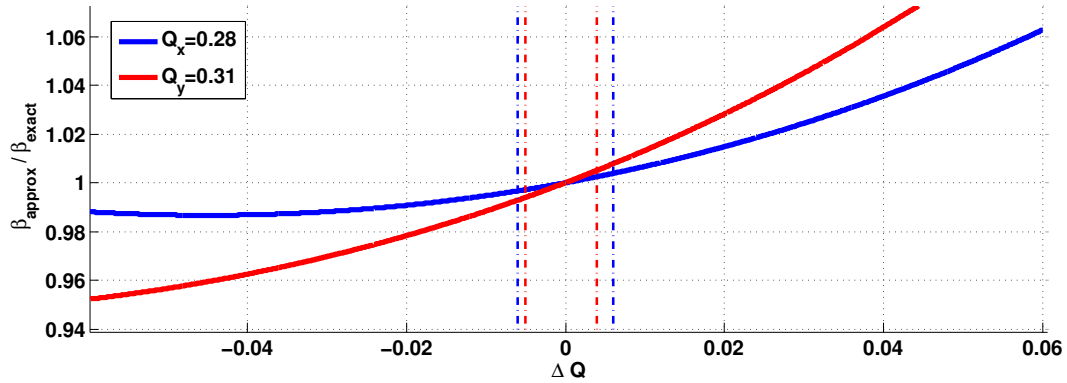
Figure 7.4: Validation of the approximation in Eq. 7.13 for the LHC parametr. The blue and red curves denote respectively the relative error introduced by the approximation in function on the induced tune change for the horizontal and vertical tune working points (0.28 and 0.31)
