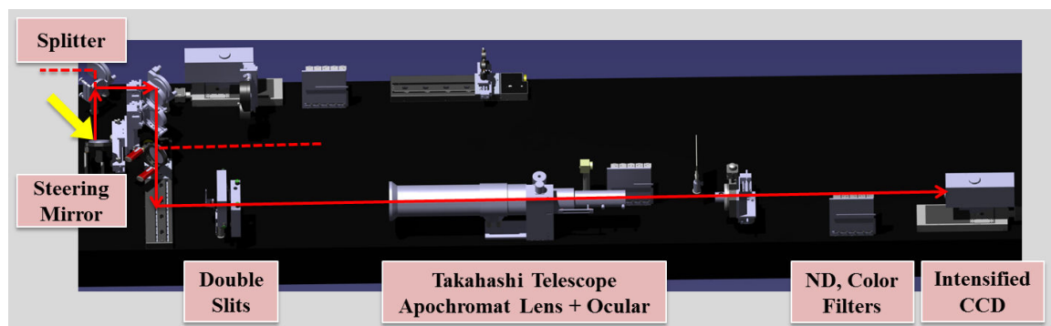
Figure 8.3: Sketch of the interferometry line to be installed in the LHC (Courtesy: A. Goldblatt).
