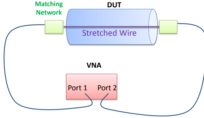
Figure 6.11: Stretched Wire technique for coupling impedance measurement.
