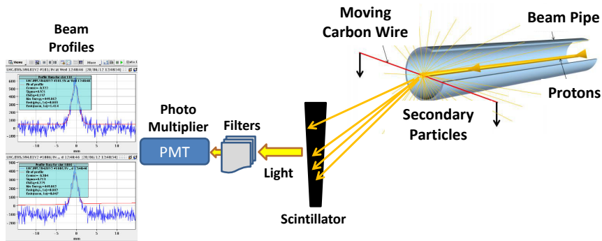
Figure 1.7: Wire Scanners working principle.
