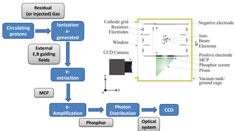
Figure 1.6: Beam Gas Ionisation monitors working principle.
