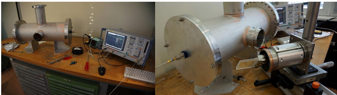
Figure 6.12: Laboratory setup for wire measurements.
