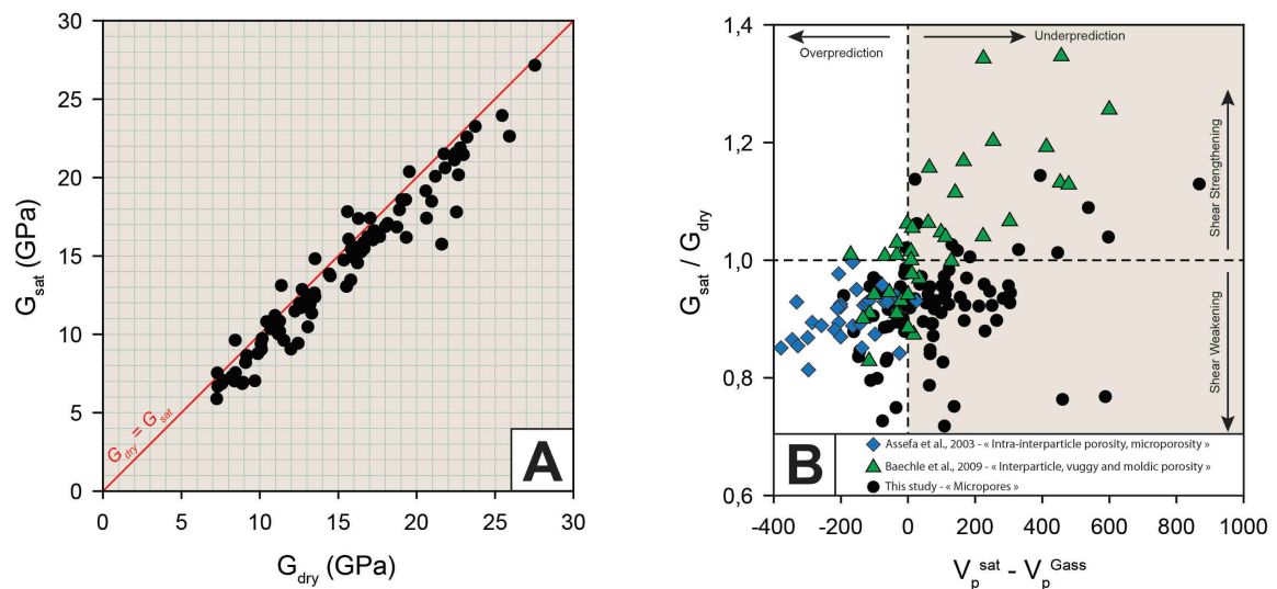
FIGURE 54 – A - Crossplot of dry shear modulus versus water-saturated shear modulus. Data points are not far away from the one-to-one straight line. B - Plot of changes in shear modulus versus the difference between measured and Gassmann-predicted velocity. Gassmann underestimates the velocities in samples with shear strengthening and overestimates the velocities in samples with shear weakening.
