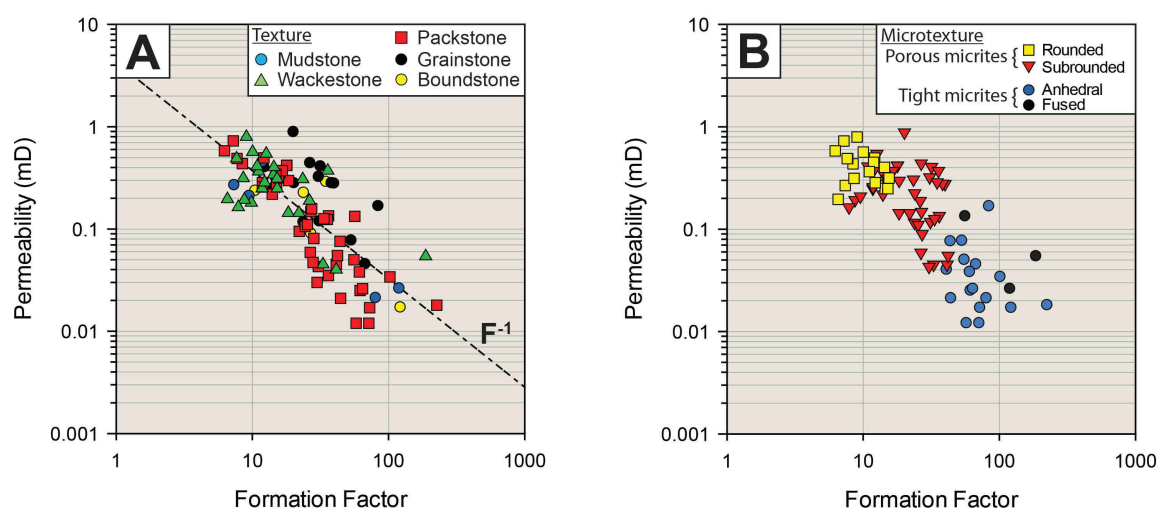
FIGURE 49 – Permeability vs. formation factor plot in log-log scale, sorted by textures (A) and micrite microtextures (B). The dashed line corresponds to the best fit (power law with exponent -1 ).
