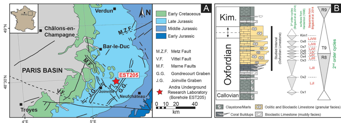
FIGURE 40 – A - Location of the study area on a geological map of the eastern part of the Paris Basin. B - Simplified Oxfordian stratigraphic column of the eastern part of the Paris Basin with main argillaceous formation bounding Oxfordian aquifer (modified from Guillocheau et al., 2000; Carpentier et al., 2014; and Brigaud et al., 2014; Thicknesses not to scale).
