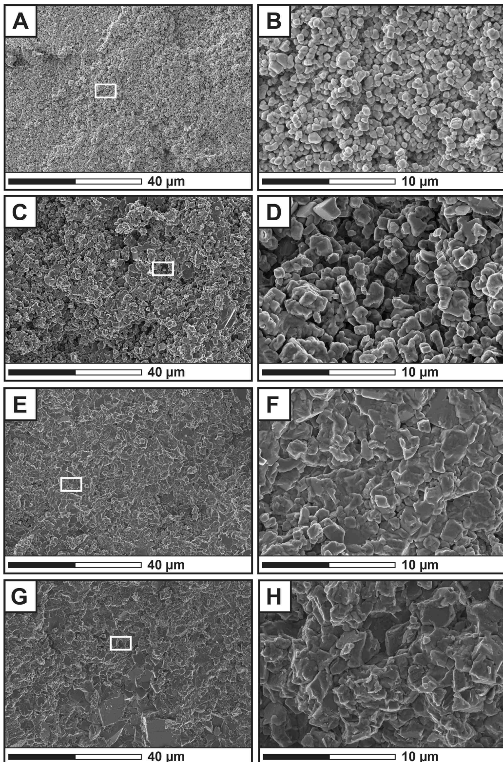
FIGURE 43 – Examples of micrite microtextures observed on SEM. White rectangles are the magnification areas. A & B - Rounded micrite from a micritic ooid grainstone ( \Phi : 19% ; 240.05 m). C & D - Subrounded micrite from a bioclastic wackestone ( \Phi : 15.6% ; 234 m). E & F - Anhedral compact micrite from a peloidal packstone ( \Phi : 5.46% ; 191.56 m). G & H - Fused micrite from oncoïd-peloid packstone ( \Phi : 2.12% ; 156.18 m).
