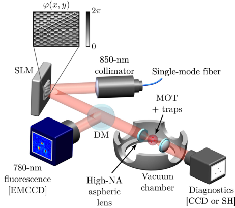
FIG. 1. Generation of an array of microtraps for single-atom trapping. The SLM imprints the calculated phase pattern \varphi(x, y) on the 850-nm dipole-trap beam. A high-numerical-aperture aspheric lens under vacuum focuses it at the center of a MOT. The intensity distribution in the focal plane is \propto |\text{FT}(A_0 e^{i\varphi})|^2 , where A_0 is the initial Gaussian amplitude profile of the 850-nm beam and FT stands for Fourier transform. The atomic fluorescence at 780 nm is reflected off a DM and detected using an EMCCD camera. A second aspheric lens (identical to the first one) recollimates the 850-nm beam. This transmitted beam is used for trap diagnostics (either with a diagnostics CCD camera or a SH wave-front sensor).
