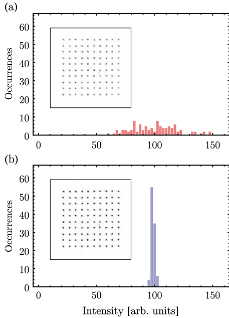
FIG. 9. Improving the uniformity of trap depths in a 10 \times 10 square array. (a) Histogram of the maximal intensity levels of the microtraps I_i , measured with the diagnostics CCD camera (see the inset), for the trap array obtained after a single use of the GS algorithm and a target image where all traps have the same intensity. The standard deviation is 19%. (b) Same as (a) but after the closed-loop optimization of the uniformity of the trap intensities. The standard deviation is now 1.4%.
