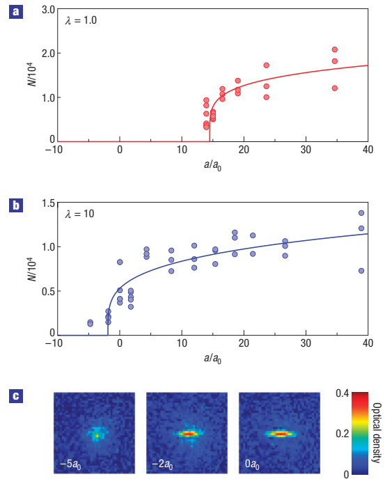
Figure 2 Decrease of the BEC atom number N around the critical scattering length a_{\text{crit}} . a,b , The critical point depends strongly on the aspect ratio \lambda of the trap. The solid lines are fits to equation (2) used to determine the critical scattering length a_{\text{crit}} (see text). c , Typical images of the atomic cloud around the critical scattering length for the trap with \lambda = 10 .
