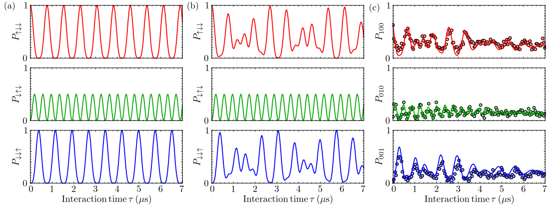
FIG. 3 (color online). Spin excitation transfer along a chain of three Rydberg atoms with nearest-neighbor separation of 20\text{ }\mu\text{m} . (a) Theoretical dynamics for a system initially prepared in |\uparrow\downarrow\downarrow\rangle , and evolving under a Hamiltonian similar to (1), but with only nearest-neighbor interactions. (b) The same as (a), but for the full Hamiltonian (1), including long-range interactions. (c) Experimental data (points) and prediction of the model taking into account experimental imperfections (see text), with no adjustable parameters. For perfect preparation and readout, the probabilities P_{\uparrow\downarrow\downarrow} (respectively, P_{\downarrow\uparrow\downarrow} , P_{\downarrow\downarrow\uparrow} ) and P_{100} (respectively, P_{010} , P_{001} ) would coincide.
