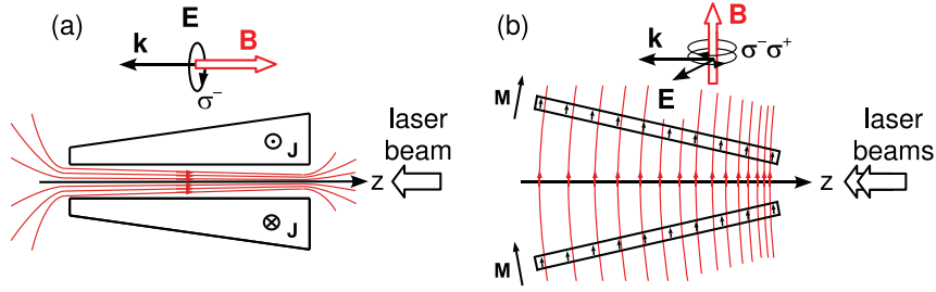
FIG. 1. (Color online) Zeeman slower configurations. (a) Conventional wire-wound tapered solenoid; magnetic field is longitudinal, \sigma^- light is used. J denotes the current density vector. (b) Use of long tilted permanent magnets; magnetic field is transverse. Light polarisation is decomposed in its \sigma^\pm components and a repumper is needed. M denotes the magnetization of the material.
