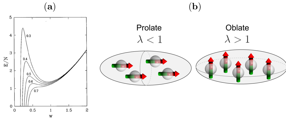
Figure 1.4: (a): Variational approach to the stability of a spherical, contact-interacting BEC. The energy of the condensate, obtained by inserting into the Gross-Pitaevskii energy functional a Gaussian trial wavefunction of size w , is plotted as a function of w for various values of the parameter N|a|/a_{\text{ho}} . Beyond a certain value, the local minimum that existed at finite w (corresponding to a metastable condensate) vanishes, indicating that the condensate collapses. (b): Intuitive picture of the geometry-dependent stability of a dipolar BEC: in a prolate (i.e. cigar-shaped, \lambda \ll 1 ) trap with the dipoles oriented along the weak axis of the trap, the attractive part of the DDI destabilizes the condensate, even in the presence of a small, positive scattering length. On the contrary, in an oblate (i.e. pancake-shaped, \lambda \gg 1 ) trap with the dipoles perpendicular to the plane, the dipoles essentially repel each other, and the condensate is stable even for a small negative scattering length.
