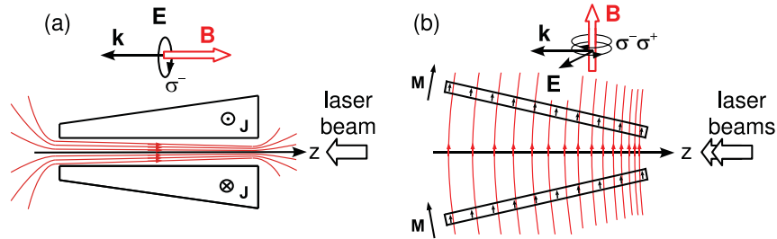
FIG. 1. (Color online) Zeeman slower configurations. (a) Conventional wire-wound tapered solenoid; magnetic field is longitudinal, \sigma^- light is used. \mathbf{J} denotes the current density vector. (b) Use of long tilted permanent magnets; magnetic field is transverse. Light polarisation is decomposed in its \sigma^\pm components and a repumper is needed. \mathbf{M} denotes the magnetization of the material.
