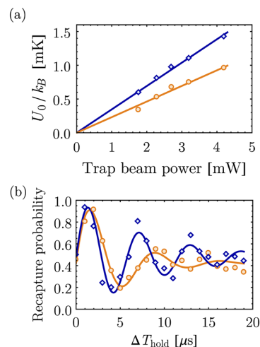
FIG. 8. (a) Trap depth U_0/k_B as a function of the trap power, with (blue diamonds) and without (orange disks) Shack-Hartmann correction. With the latter, the trap depth increases by about 50%. (b) Recapture probabilities for an atom oscillating in the trap as a function of the hold time \Delta T_{\text{hold}} . The trap frequency increases by about 30% when the Shack-Hartmann correction pattern is added to the SLM.
