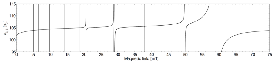
Figure 1.2: Scattering length for two chromium atoms as a function of the applied magnetic field. Figure taken from [130]. Note the limited scale of the y -axis.
