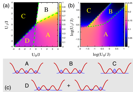
FIG. 2 (color online). (a) \langle \hat{n} \rangle/N as a function of U_{0,1} for N = 18 . (b) \Delta \hat{\delta}/N in logarithmic scale for U_{0,1} . The dashed lines show the boundaries between the classical phases (A)–(D) that are shown schematically in (c).
