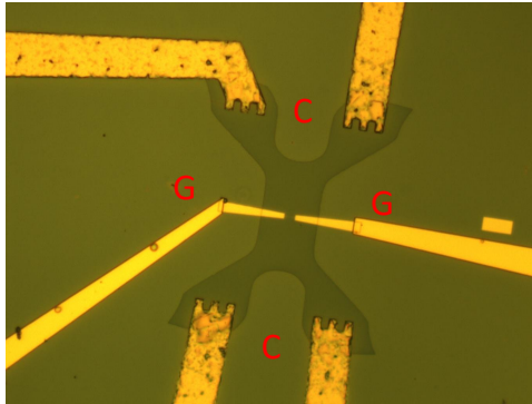
FIGURE B.7 – Label G and C are respectively Gates and Ohmic contacts. Mesa, contacts and gate pattern are inherited from the work of Bajjani et al. [7][156]. The split-gate is too thin near the tip end to be observed. Real size : 120x200 \mu\text{m} .
