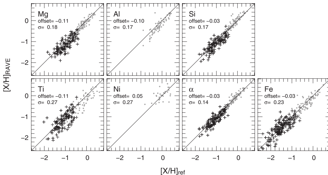
Figure 16. Comparison between the reference high-resolution elemental abundances (x-axis) and RAVE elemental abundances (y-axis) for the SG05 (98 dwarf stars, gray dots) and the R11 samples (233 spectra of 203 giant stars, black “+”) measured by adopting the stellar parameters provided by the RAVE pipeline.
