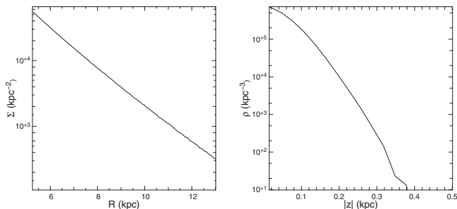
Figure 2. Initial conditions. Left-hand panel: number of stars per \text{kpc}^2 (surface density) within the Galactic plane as a function of R . Right-hand panel: stellar density as a function of z at R = 8 kpc.
