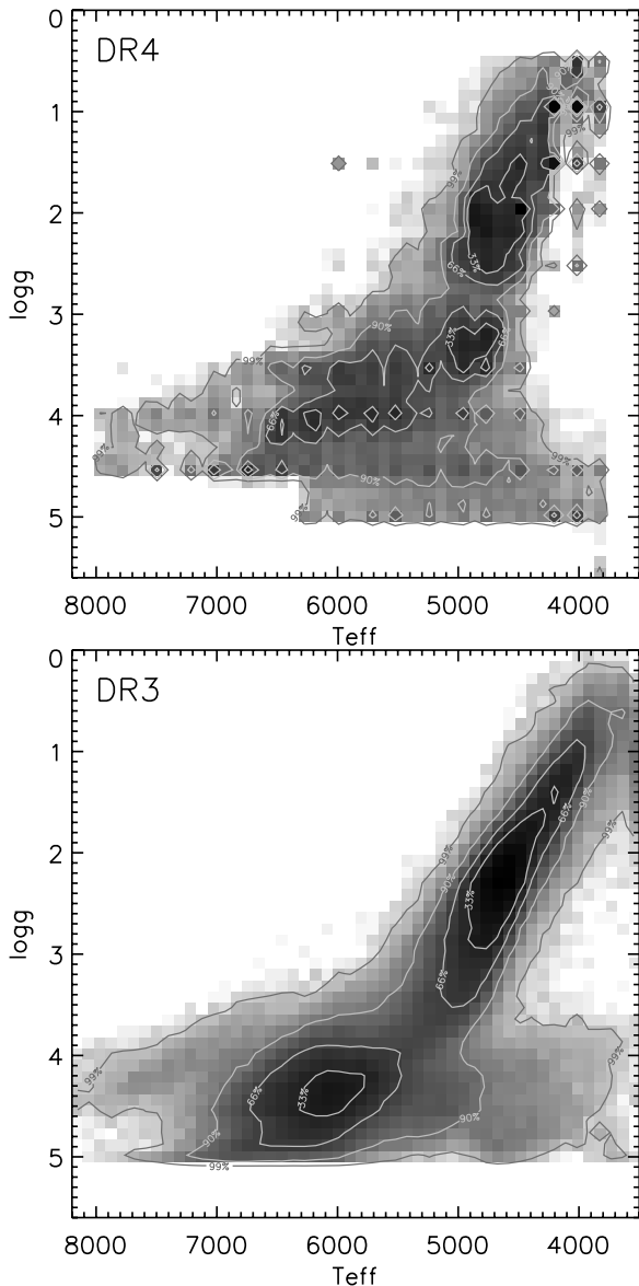
Figure 20. T_{\text{eff}}-\log g diagram for the selected RAVE stars (top: DR4 pipeline; bottom: DR3 pipeline), meeting our criteria defined in Section 6.1. In total the parameters of \sim 4 \times 10^5 spectra are represented in these diagrams. The contour lines contain 33%, 66%, 90%, and 99% of the total considered sample.
