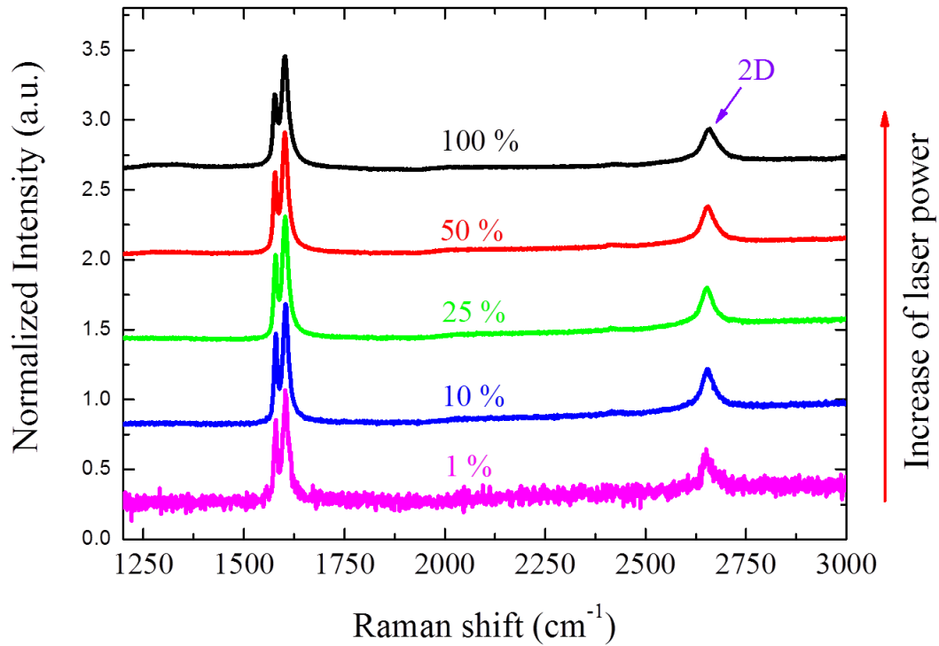
Figure 3A: Raman spectra of laser induced deintercalation for stage-3 \text{KC}_{36}
