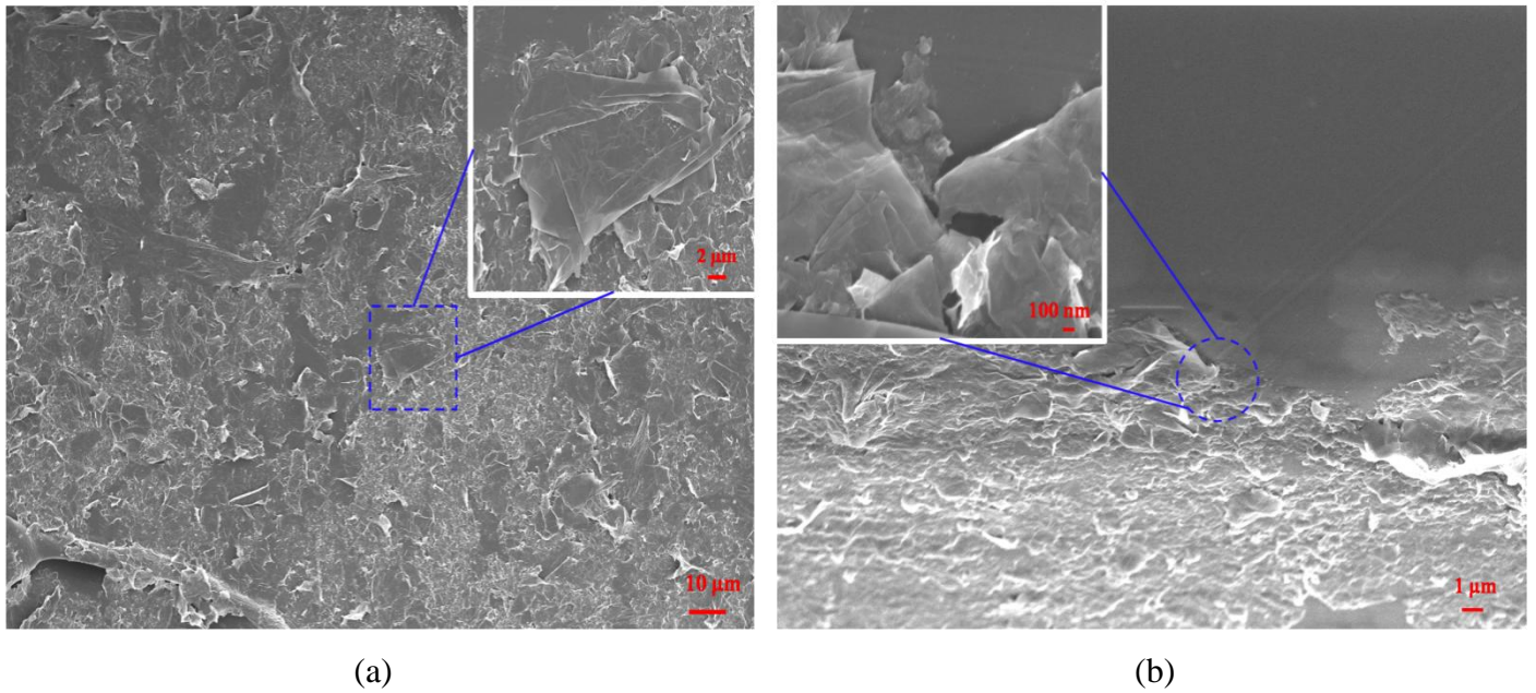
Figure 4.5: SEM of graphene film on \text{Al}_2\text{O}_3 substrate. (a) centre of film; (b) edge of film.
