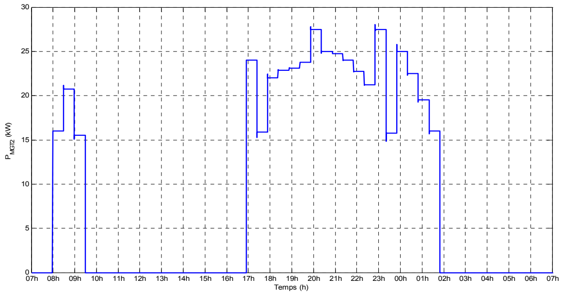
Fig. 4.26. P_{MGT\_2}
