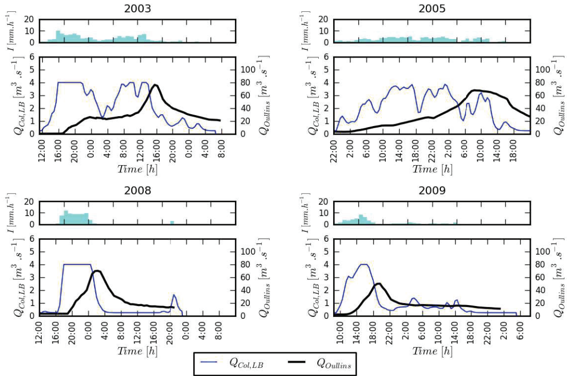
Figure 7.4 : Rainfall intensity I , Zeron flow discharge at Oullins Q_{Oullins} and main collector flow hydrograph Q_{Col,LB} just upstream of the modelled area (computed with the rainfall-runoff model) for the 4 studied flood events
