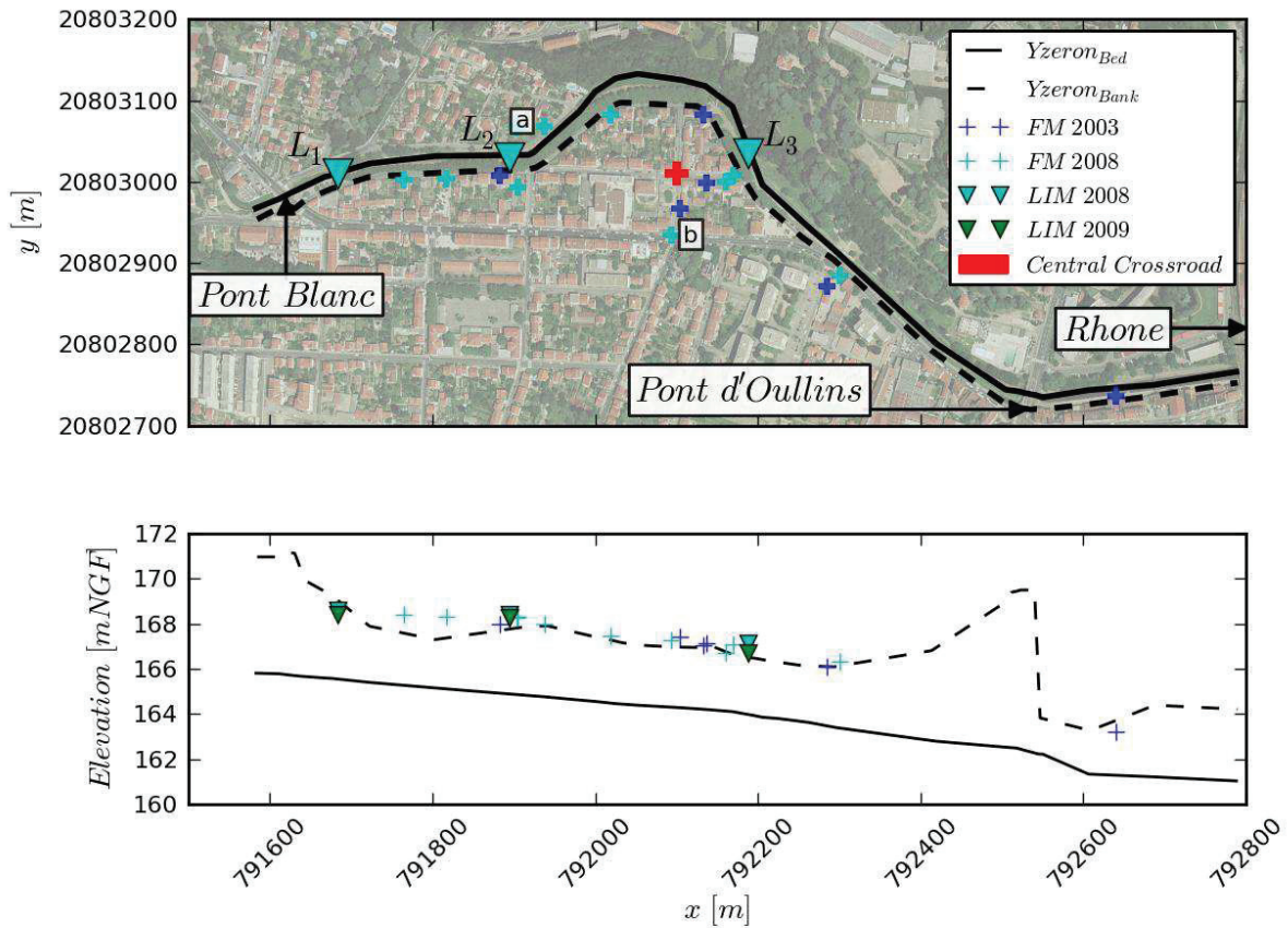
Figure 6.3 : Top view of the flooded area with recorded flood marks (FM) and stage gauges (LIM). View along x-axis of the river bed elevation (Yzeron Bed ), right bank elevation (Yzeron Bank ), recorded flood marks and maximum water levels at the stage gauges.
