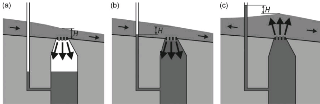
Figure 4.1: Types of exchange flows depending on hydraulic configurations through a schematic exchange structure: free drainage (a), influenced drainage (b) and overflow (c). From (Djordjevic et al. 2005)
