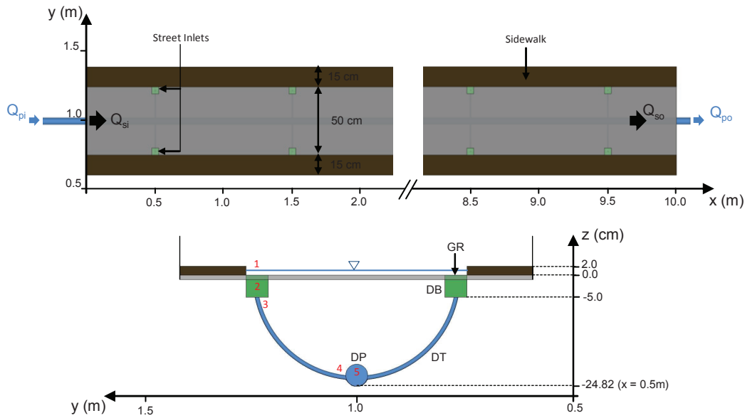
Figure 4.3 : Top view and cross section view (at x = 0.5\text{m} ) of the experimental facility with its main dimensions. The drainage structure elements are indicated in upper case: street inlet grid (GR), drainage box (DB), drainage tube (DT) and drainage pipe (DP). The street level is at z=0 .
