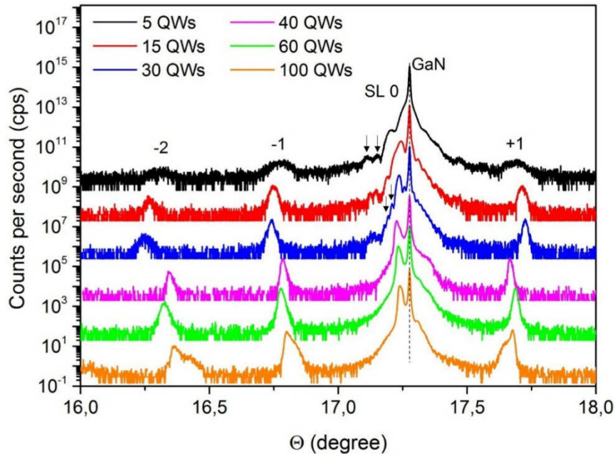
Figure 4.2. X-ray \omega - 2\theta scan around (0002) Bragg peak reflection at 1.54056 Å wavelength for samples with 5-100 \times In 0.1 Ga 0.9 N( \sim 2 nm)/GaN( \sim 8 nm) QWs. Arrows show the thickness fringes.
