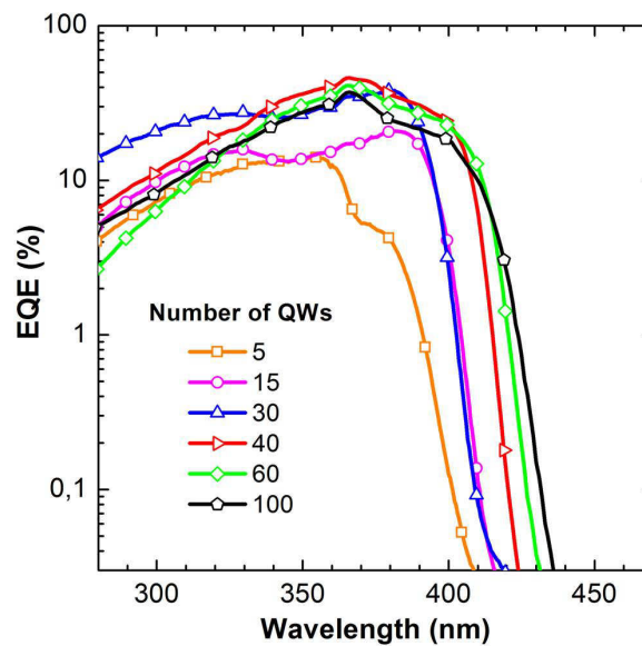
Figure 4.13. Spectral response of the \text{In}_{0.11}\text{Ga}_{0.89}\text{N}(1.7 \text{ nm})/\text{GaN}(8\text{-}9 \text{ nm}) samples varying the number of quantum wells [Valdúeza, 2013].
