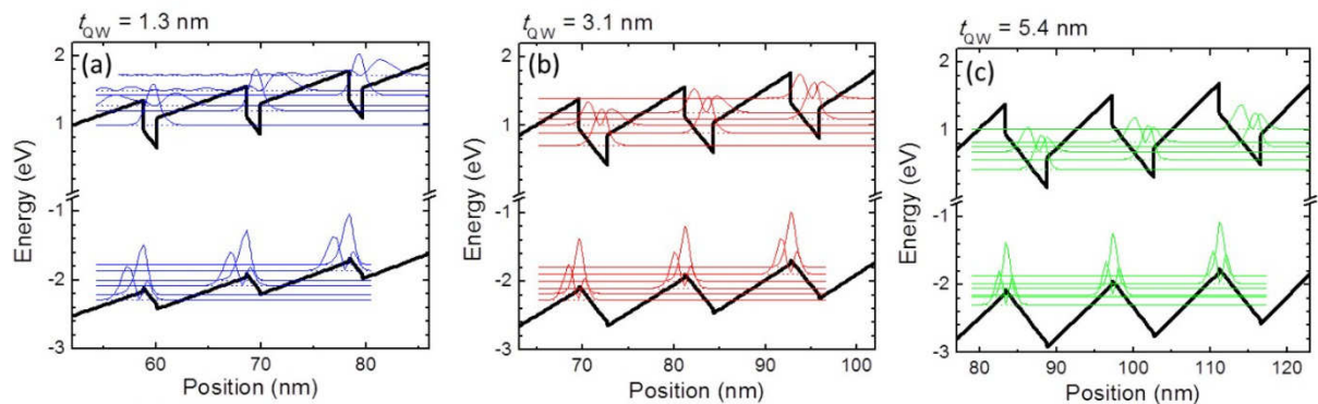
Figure 5.2. Band diagrams of the \text{In}_{0.12}\text{Ga}_{0.88}\text{N}/\text{GaN} ( t_{\text{QW}} / 8.5 nm) MQW structure for (a) t_{\text{QW}} = 1.3 nm, (b) t_{\text{QW}} = 3.1 nm, (c) t_{\text{QW}} = 5.4 nm. Two first electronic levels in each QW are shown with their squared wave functions [Redaelli, 2014].
