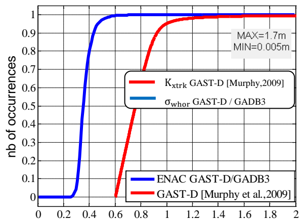
Figure 93: Comparison between observed \sigma_{whor} CDF for GAST-D/GAD B3 using ENAC mean probabilities and K_{xtrk} generation function from [Murphy et al., 2009]
