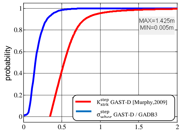
Figure 97: Comparison between observed nominal \sigma_{whor}^{step} CDF for GAST-D and GAD B3 using ENAC mean probabilities and K_{xtrk}^{step} generation function from [Murphy et al.,2009] for GAST-D
