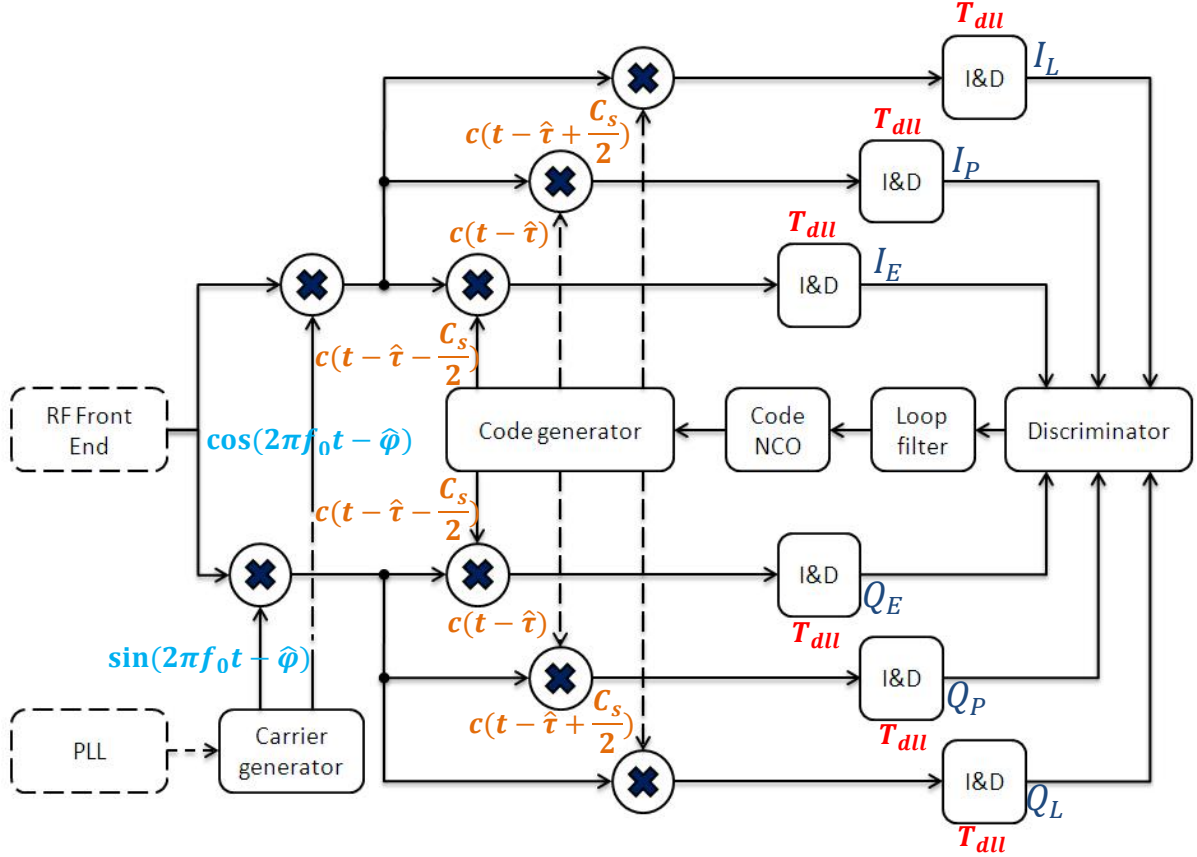
Figure 9: Structure of a classic DLL (with T_{au} the correlator integration time)
