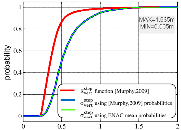
Figure 87: Comparison between observed faulted \sigma_{vert}^{step} CDF for GAST-C and GAD B3 and K_{vert}^{step} generation function from [MURPHY, 2009]
