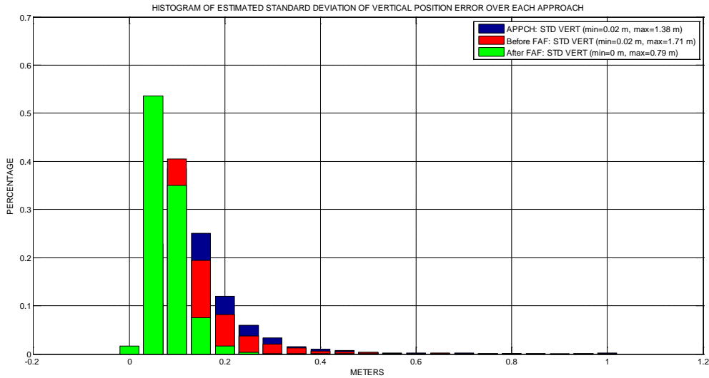
Figure 55: Comparison of histograms of estimated std of VPE over all simulation runs before and after the FAF with constellation freezing algorithm
