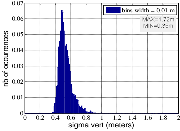
Figure 69: observed \sigma_{vert} histograms for GAST-C and GAD B3
