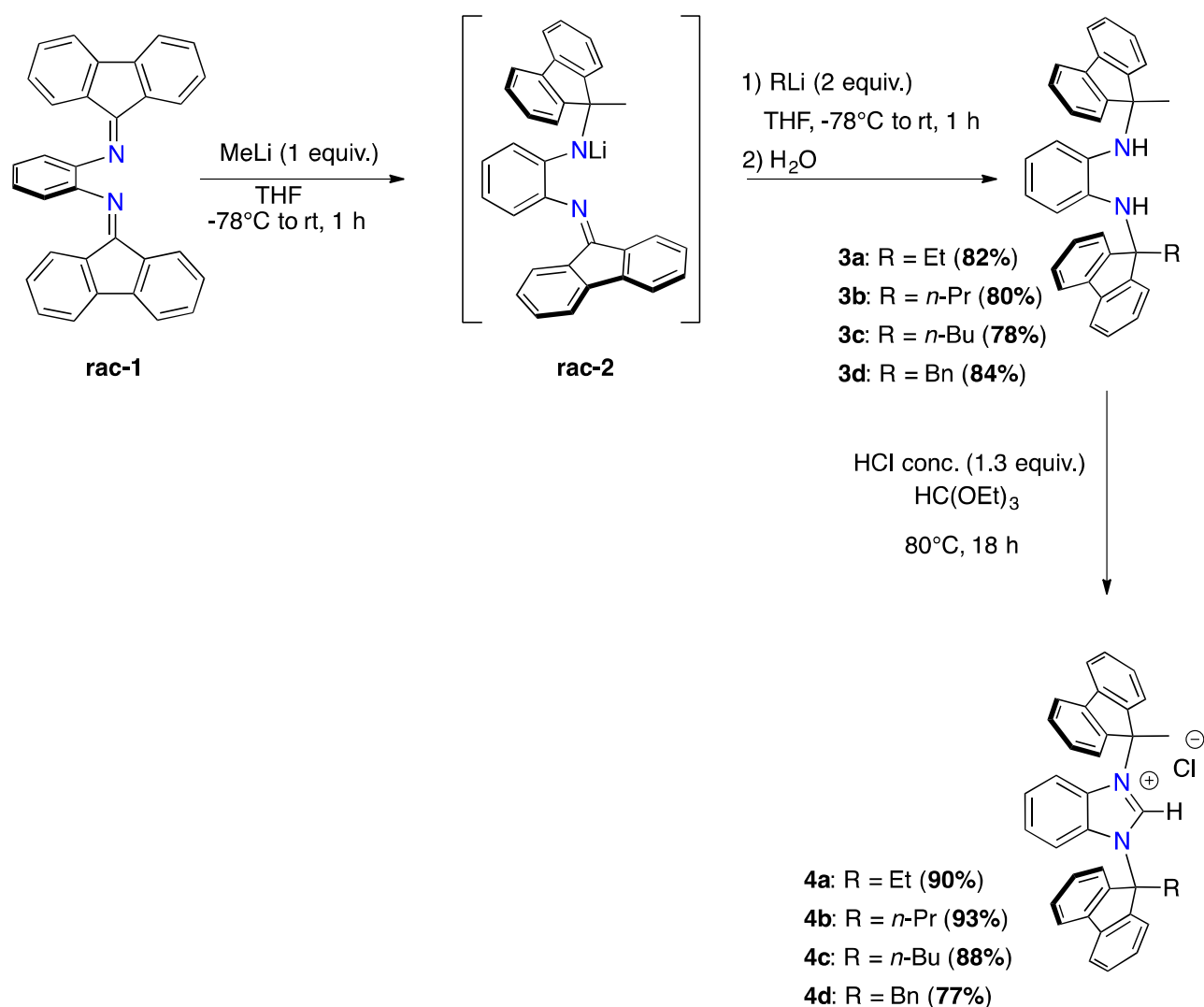
Scheme 1: Synthesis of benzimidazolium salts 4a-d
