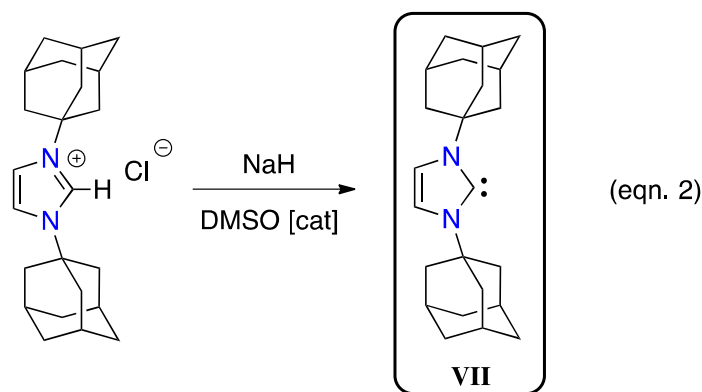
Scheme 5: Synthesis of the first stable free carbenes.
