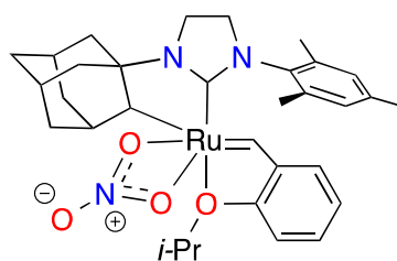
Figure 18: Grubbs Z -selective olefin metathesis catalyst.
