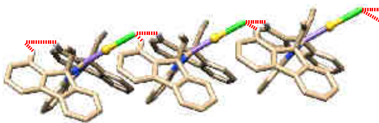
Figure 2: Supramolecular chain structure of 3 in the solid state
