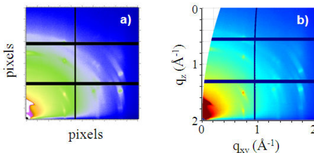
Figure 2.17: Example of conversion of a a) 2D-GIXRD image as visualized on the detector to b) the correct representation of the reciprocal space probed.
