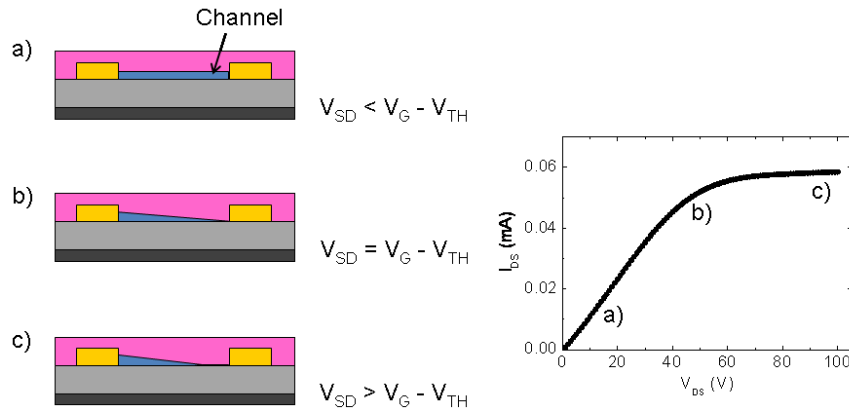
Figure 1.14: Operating regimes in OFETs: the current first linearly increases with V_{SD} then gradually saturates approaching a constant value.
