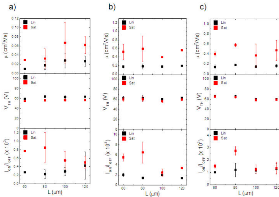
Figure 4.9: Electrical results of a) \sim 1 ML, b) \sim 2 MLs and c) \sim 3 MLs of N2200 thin-films deposited by LS technique on OTS-treated substrate and annealed at 150 ^{\circ}\text{C} overnight in vacuum oven.
