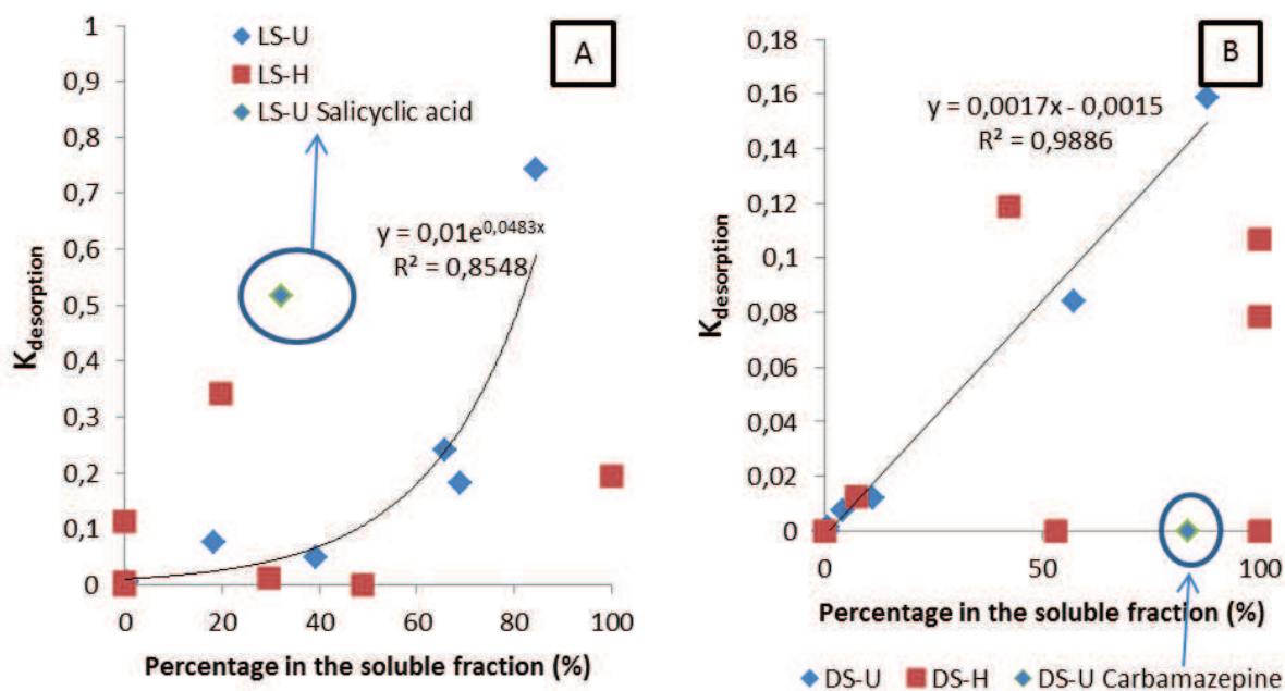
Figure 94 : Relation between K_{\text{desorption}} and the percentage in the soluble phase for the different pharmaceutical compounds in limed sludge (LS, fig A) and digested sludge (DS, fig B)
