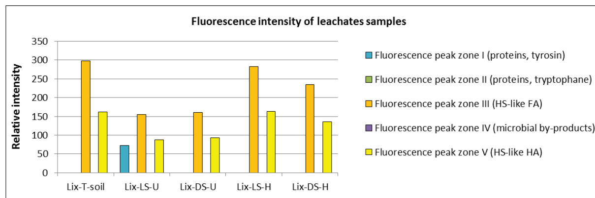
Figure 97 : Fluorescence relative intensity of leachates samples
