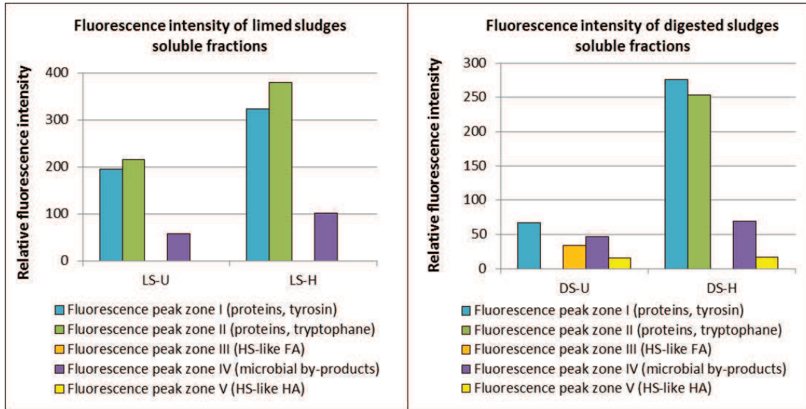
Figure 95 : Fluorescence of the soluble phases of limed and digested sludge. Comparison between urban and hospital origins
