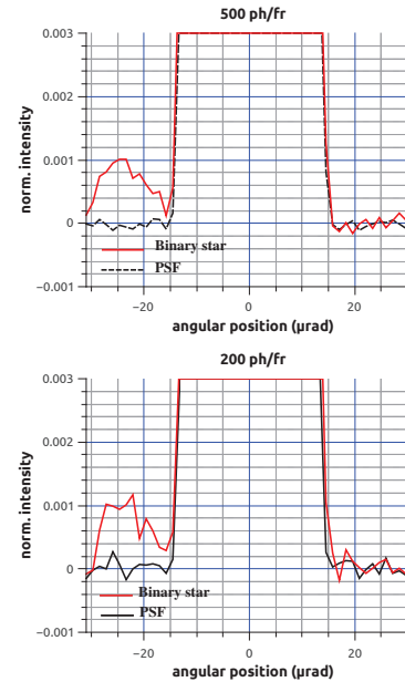
Fig. 13. Experimental images of a single star and a binary star obtained with the THT test bench in the photon-counting regime. Two photon flux are investigated (top: 500 and bottom: 200 photons/frame). The number of pixels is equal to 50 across the clean field of view. These images are obtained by stacking 30 000 and 20 000 short-exposure images for 200 and 500 ph/fr respectively. The intensity ratio between the two components of the unbalanced binary star is set to 1:1000 and their angular separation is 25 \mu rad. The dynamic range (DR) of each long-exposure PSF measured before the background bias subtraction are close to 450 and 730 for 200 and 500 ph/fr, respectively.
