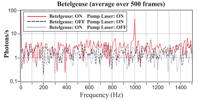
Figure 3. Frequency conversion of Betelgeuse (MMag = -3.9 in the H band). Red solid line: Betelgeuse and the pump source on. Black dashed line: Betelgeuse off and the pump source on. Blue dotted line: Betelgeuse on and the pump source off.
