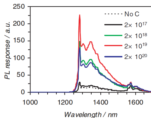
Figure 2. Photoluminescence spectra measured at 80 K of silicon samples implanted with different carbon doses and annealed at 1000 °C for 20 s, followed by proton irradiation at 5 \times 10^{13} cm^{-2} at 2 MeV. The carbon concentrations ( cm^{-3} ) are indicated.
