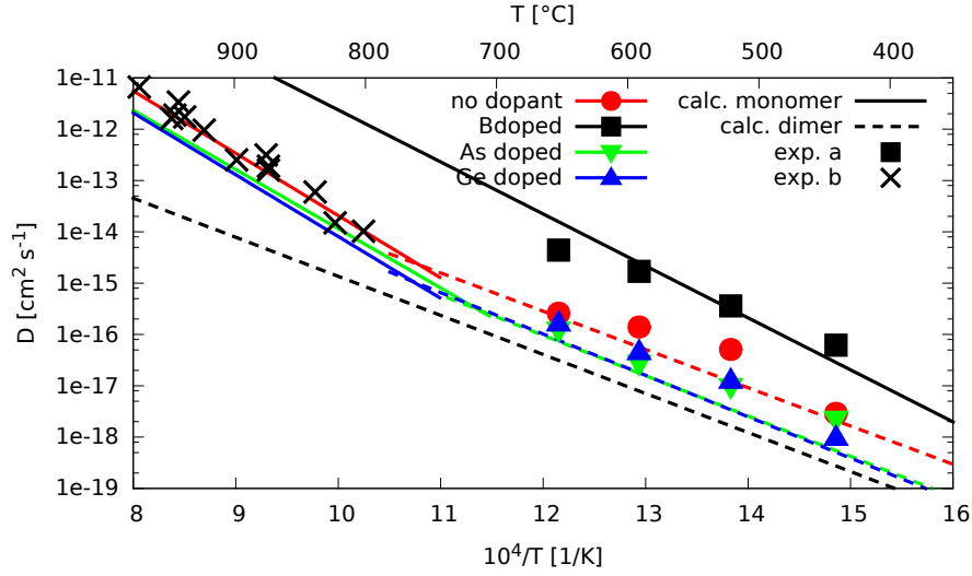
Figure 4.13: Calculated diffusion coefficients of oxygen monomers and dimers. [a] Reference [60]; [b] Reference [117].
