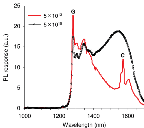
FIG. 1. Photoluminescence spectra, observed at 80K, of pre-amorphised silicon samples A03 and A05 ( 2 \times 10^{20} C cm^{-3} irradiated with 5 \times 10^{13} and 5 \times 10^{15} H^+ cm^{-2} , respectively). The positions of the G- and C-centres are also shown.
