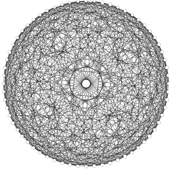
Figure 5.5: Adjacency graph of a GQ(3, 5).
