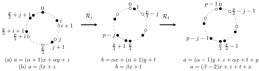
Figure 6.18: Rotations of the colouring c of a Type2mod cycle with c(j+1) \neq c(\frac{p}{2} + j + 1) = 0 , and their corresponding weighted sums of black vertices which are not all equal, where the line (a) corresponds to the case x \neq y and the line (b) to the case x = y .
