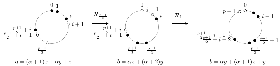
Figure 6.9: Rotations of the colouring c of a Type1mod cycle with c(j) = 1 for all 0 \leq j \leq i with i > 1 , and their corresponding weighted sums of black vertices distinct which are not all equal.
