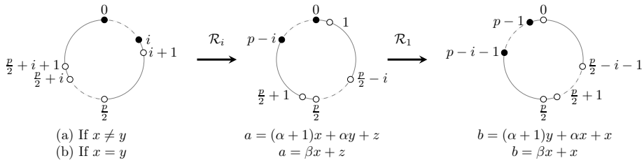
Figure B.13: Rotations of the colouring c of a Type4mod cycle and their corresponding weighted sums of black vertices depending on the equality of the weights x and y .
