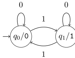
Figure 1.1: A deterministic finite automaton with output (DFAO).
