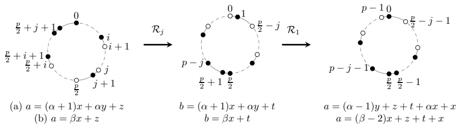
Figure B.14: Rotations of the colouring c of a Type4mod cycle with c(j+1) \neq c(\frac{p}{2}+j+1) = 0 , and their corresponding weighted sums of black vertices which are not all equal, where the line (a) corresponds to the case x \neq y and the line (b) to the case x = y .
