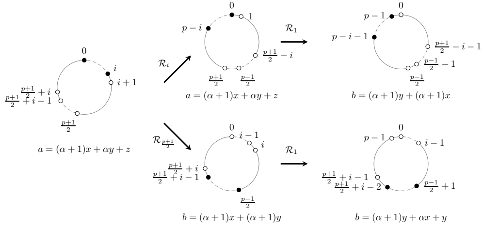
Figure 6.7: Rotations of the colouring c of a Type1mod cycle with c(\frac{p+1}{2} + i) = 0 , and their corresponding weighted sums b of black vertices which are not all equal.
