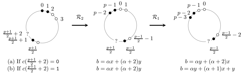
Figure 6.10: Rotations of the colouring c of a Typelmod cycle with c(0) = c(1) = 1 , c(\frac{p+1}{2} + 1) = 1 and c(3) = c(\frac{p+1}{2}) = 0 , and their corresponding weighted sums of black vertices depending on the colour c(\frac{p+1}{2} + 2) .
