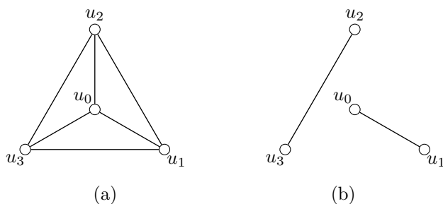
Figure 4.2: A graph (a) and one of its perfect matchings (b).
