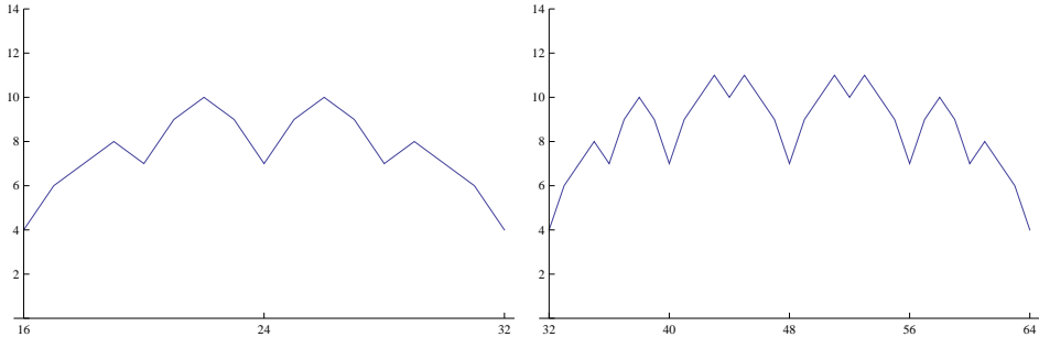
Figure 2.9: The abelian complexity of \text{block}(\mathbf{p}, 2) on the intervals [16, 32] and [32, 64] .
