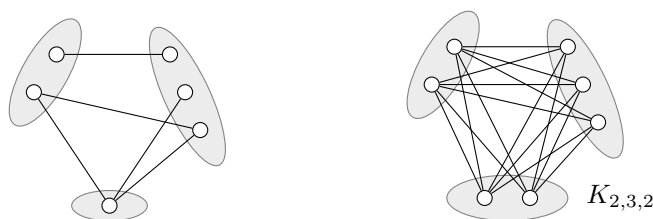
Figure 4.3: Two 3-partite graphs.
