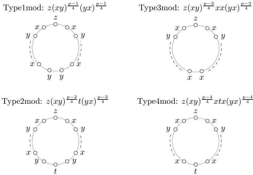
Figure 6.3: Types of weighted cycles \mathcal{C}_p .
