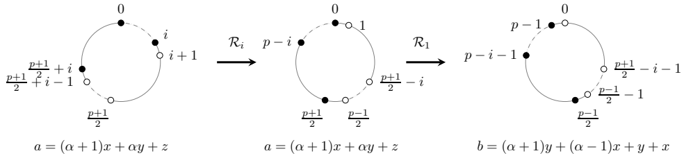
Figure 6.8: Rotations of the colouring c of a Type1mod cycle with c(\frac{p+1}{2} + i) = 1 , and their corresponding weighted sums of black vertices.
