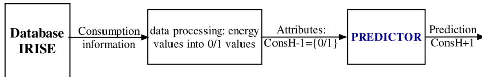
FIGURE 8.8 – Simple prediction architecture with no expert knowledge addition.
