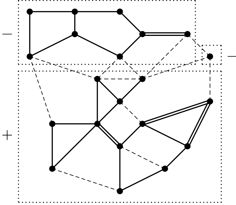
Fig.4.1: Full lines are the edges visited by discrete loops. Double lines are additionally opened edges. Dashed lines are edges left closed. Dotted contours surround clusters in \mathfrak{C}' .
