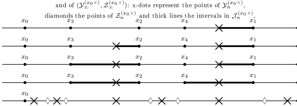
Fig.3.2.a - Illustration of the first four steps of Wilson's algorithm in case of killing at x_0
