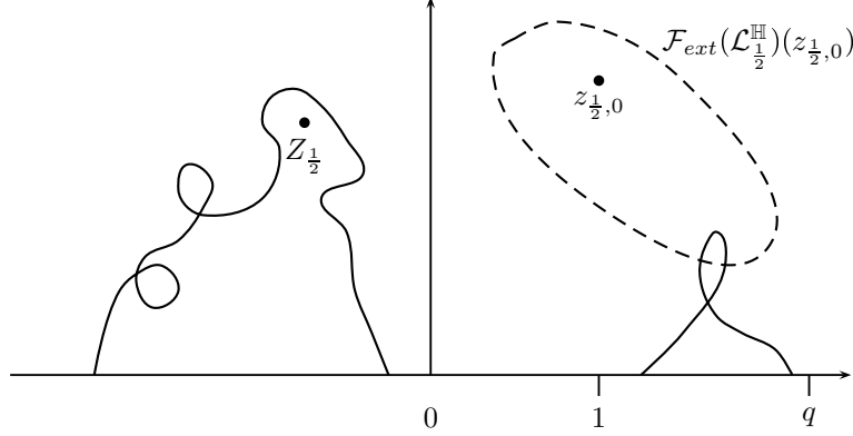
Fig. 5.5: Illustration of A_{\frac{1}{2},u,v}^+(q) where an excursion from \mathcal{E}_u^H((-\infty, 0]) surrounds Z_{\frac{1}{2}} and an excursion from \mathcal{E}_v^H([1, q]) intersects \mathcal{F}_{ext}(\mathcal{L}_{\frac{1}{2}}^H)(z_{\frac{1}{2},0}) .
