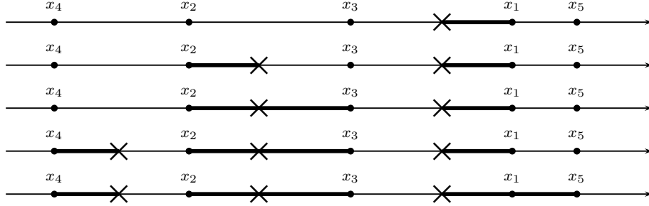
Fig.3.1.a - Illustration of ((\mathcal{V}_n, \mathcal{J}_n))_{1 \leq n \leq 5} : x-dots represent the points of \mathcal{V}_n and thick lines the intervals in \mathcal{J}_n .
