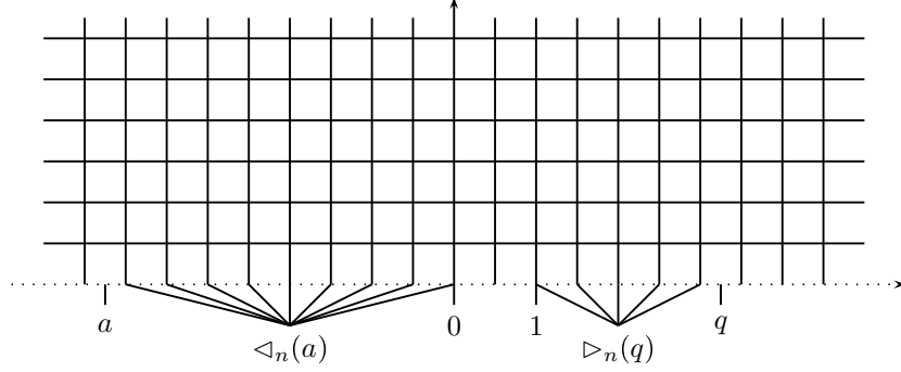
Fig.5.3: Illustration of points identified into \triangleleft_n(a) and \triangleangleright_n(q) .
