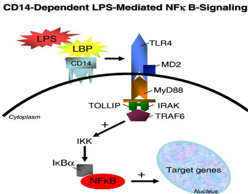
Fig.1.14 (A): Diagram illustrate the signalling interaction between CD14 and LPS (adapted from (Linde et al., 2007)).
