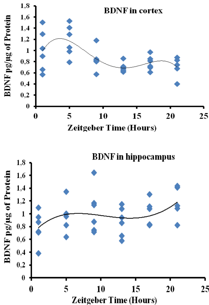
Figure1B. BDNF protein (pg/μg of protein) the prefrontal cortex and hippocampus supernatant at different Zeitgeber times (ZT1, ZT5, ZT9, ZT13, ZT17, and ZT21) in Arvicanthis ansorgei . Cosinor analysis of data of BDNF protein during 24 h shows an unimodal circadian rhythm of BDNF protein in the prefrontal cortex but not in the hippocampus.
