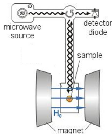
Figure IV.3 – Scheme of the FMR measurement setup
