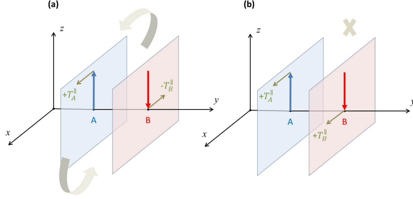
Figure II.2 – (a) Effective in-plane torque in an AF lead resulting from local torques of alternating sign from layer A (up spins) to the adjacent layer B (down spins). (b) Ineffective in-plane torque due to local torques of the same sign in adjacent layers; Heisenberg field maintains the lattice rigid and the order parameter does not change orientation.
