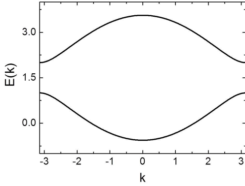
Figure II.11 – Dispersion relation within the FBZ for a 1-D AF with \epsilon_0 = 1.5 eV, \Delta = 0.5 eV and t = -1 eV. The wave vector k is in 1/a units.
