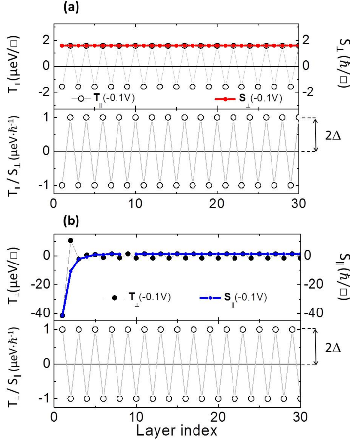
Figure III.8 – (a) (Top) Computed spatial distribution of the in-plane torque ( T_{\parallel} ) and out-of-plane spin density ( S_{\perp} ) for a 3-D AF/B/AF junction with \theta = \pi/2 , V = -0.1V , \epsilon_0 = 1.5 eV and \Delta = 0.5 eV in both AF leads. (Bottom) Local ratio T_{\parallel}/S_{\perp} showing explicitly the exchange field \Delta = 2\Delta (b) (Top) Computed spatial distribution of the out-of-plane torque ( T_{\perp} ) and in-plane spin density ( S_{\parallel} ) for the same system. (Bottom) Local ratio T_{\perp}/S_{\parallel} showing explicitly the exchange field \Delta = 2\Delta . The red and blue thick lines representing the out-of-plane and in-plane spin densities in (a) and (b) respectively refer to the right-hand ordinate.
