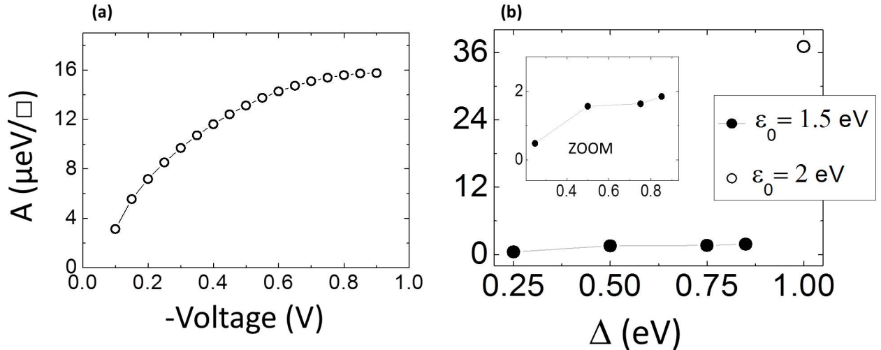
Figure III.9 – (a) Dependence of the in-plane torque amplitude A in \mu\text{eV} per unit of surface \square on the applied voltage for a 3-D AF/B/AF junction with \theta = \pi/2 and \Delta = 0.5\text{ eV} . (b) Dependence of the in-plane torque amplitude A on the spin splitting \Delta for the same junction at V = -0.1\text{V} . The inset is a zoom for the low values of the amplitude.
