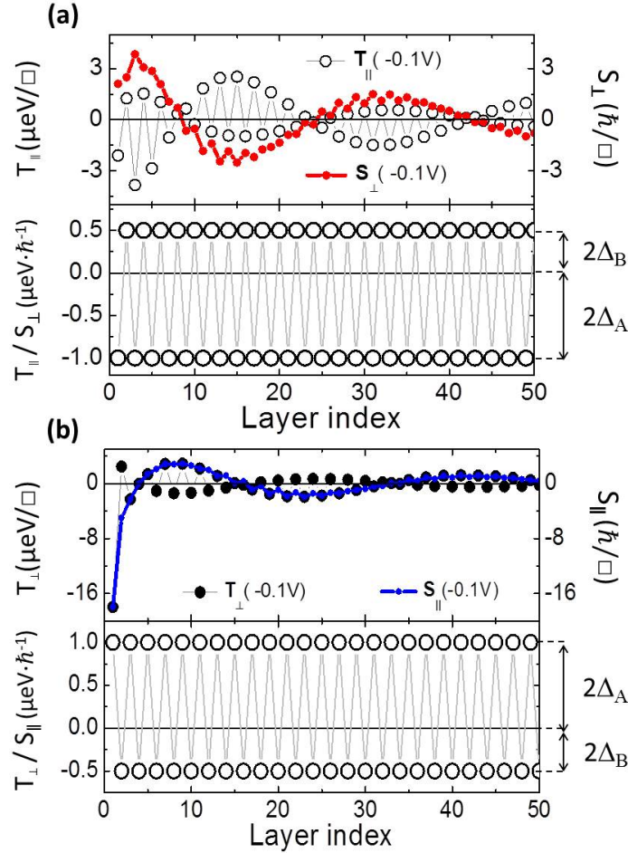
Figure III.23 – (a) (Top) Computed spatial distribution of the in-plane torque ( T_{\parallel} ) and out-of-plane spin density ( S_{\perp} ) for a 3-D FI/B/FI junction with \theta = \pi/2 , V = -0.1\text{V} , \epsilon_0 = 1.5\text{ eV} , \Delta_A = 0.5\text{ eV} and \Delta_B = 0.25\text{ eV} in both FI leads. (Bottom) Local ratio T_{\parallel}/S_{\perp} showing explicitly the exchange field \Delta_A = 2\Delta_A ; \Delta_B = 2\Delta_B (b) (Top) Computed spatial distribution of the out-of-plane torque ( T_{\perp} ) and in-plane spin density S_{\parallel} ) for the same system. (Bottom) Local ratio T_{\perp}/S_{\parallel} showing explicitly the exchange field \Delta_A = 2\Delta_A ; \Delta_B = 2\Delta_B . The red and blue thick lines representing the out-of-plane and in-plane spin densities in (a) and (b) respectively refer to the right-hand ordinate.
