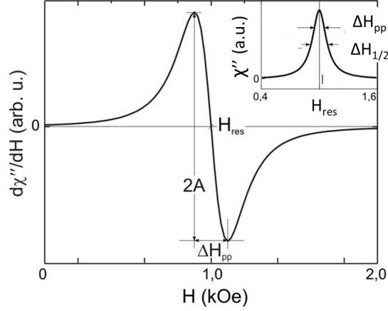
Figure IV.5 – Differential absorption \frac{\partial \chi''}{\partial H} as a function of the applied static field. The inset corresponds to the Lorentzian susceptibility \chi'' .
