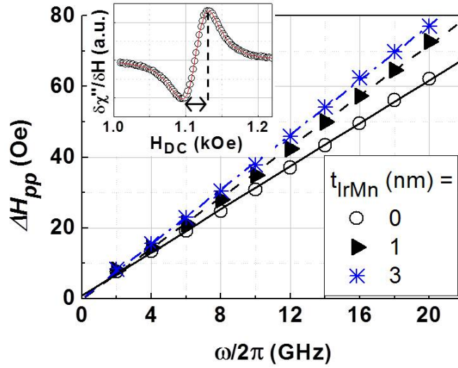
Figure IV.11 – Dependence of the resonance linewidth ( \Delta H_{pp} ) with the excitation frequencies ( \omega/2\pi ) for Si/SiO 2 //NiFe(8)/Cu(3)/IrMn( t_{\text{IrMn}} )/Al(2) (nm) stacks with t_{\text{IrMn}} = 0; 1 and 3 nm. The lines are linear fit to the data. Inset: typical resonance spectrum, i.e. differential power absorption \frac{\partial \chi''}{\partial H} VS DC bias field ( H_{\text{DC}} ) for t_{\text{IrMn}} = 1 nm and ( \omega/2\pi ) = 10 GHz; the peak-to-peak linewidth gives \Delta H_{pp} and is indicated by the arrow.
