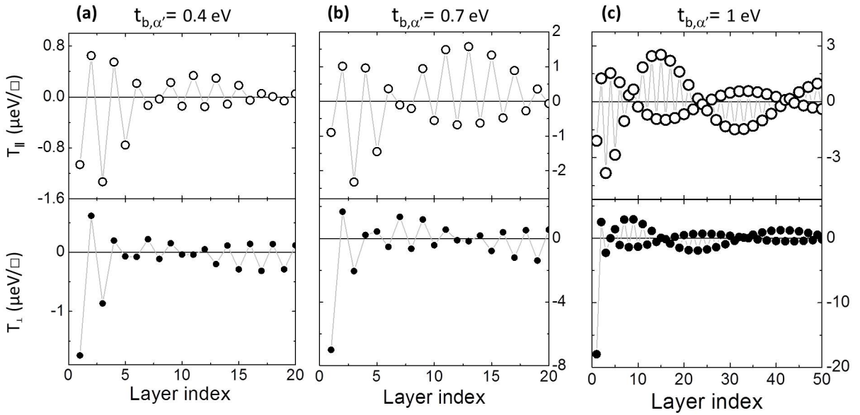
Figure III.24 – Computed spatial distributions of the in-plane ( T_{\parallel} ) and out-of-plane ( T_{\perp} ) components of the torque in \mu\text{eV} per unit of surface \square for a 3-D FI/B/FI junction with \theta = \pi/2 , V = -0.1\text{V} , \epsilon_0 = 1.5\text{eV} , \Delta_A = 0.5 eV and \Delta_B = 0.25 eV in both FI leads. The hopping parameter at the barrier interfaces (coupling) is t_{b,\alpha'} = t_{a,\alpha} = (a) 0.4 eV. (b) 0.7 eV. (c) 1 eV.
