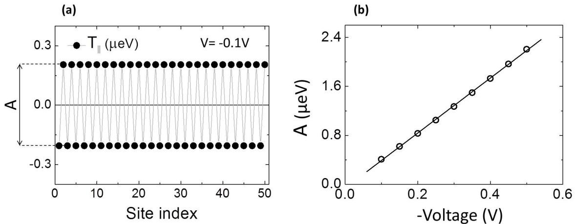
Figure III.4 – (a) Definition of the amplitude A (in \mu\text{eV} ) of the in-plane torque in a 1-D AF/B/AF junction with \theta = \pi/2 , V = -0.1\text{V} , \epsilon_0 = 1.5\text{eV} and \Delta = 0.5\text{eV} . (b) Voltage dependence of A in the same system. The line is a linear fit to the data.
