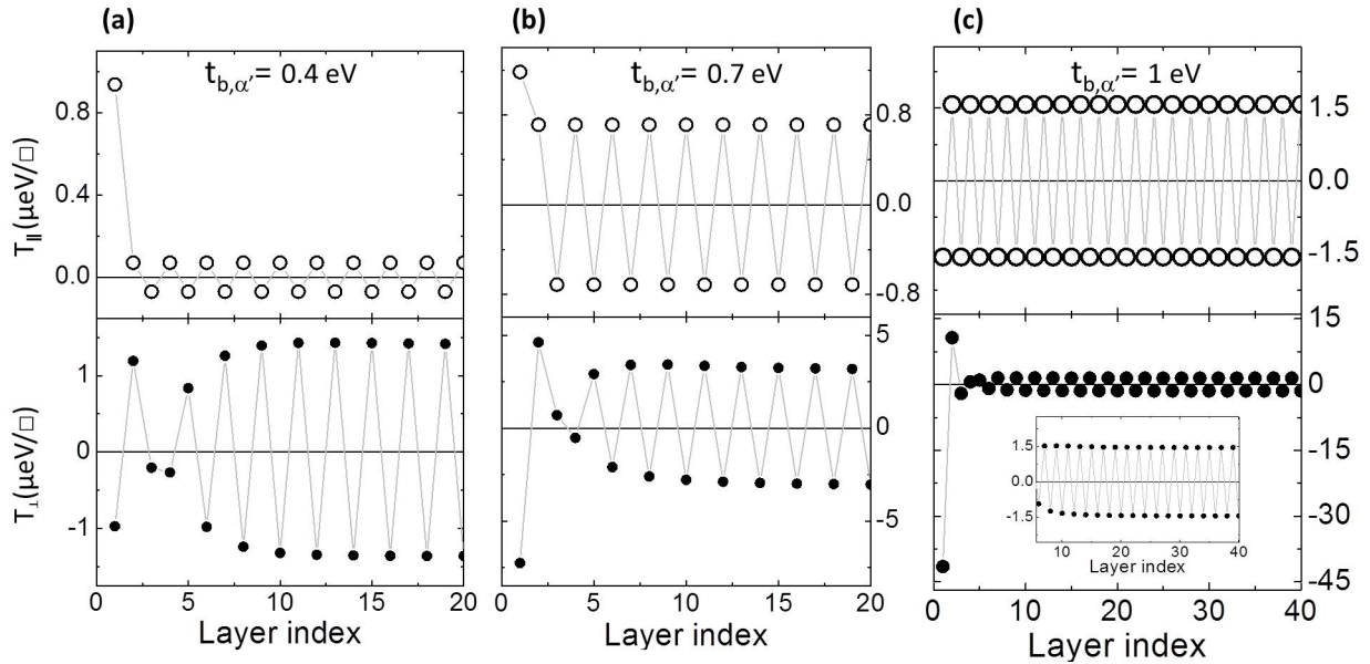
Figure III.10 – Computed spatial distributions of the in-plane ( T_{\parallel} ) and out-of-plane ( T_{\perp} ) components of the torque in \mu\text{eV} per unit of surface \square for a 3-D AF/B/AF junction with \theta = \pi/2 , V = -0.1\text{V} , \epsilon_0 = 1.5\text{eV} and \Delta = 0.5 eV in both AF leads. The hopping parameter at the barrier interfaces (coupling) is t_{b,\alpha'} = t_{a,\alpha} = (a) 0.4 eV. (b) 0.7 eV. (c) 1 eV. As in Fig. III.6, the inset is a zoom of the out-of-plane component from the sixth layer.
