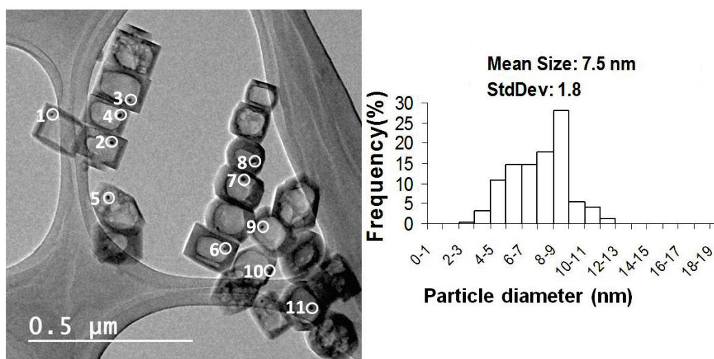
Figure 9: TEM image (left) and particle size distribution (right) of \text{Pd}_{0.21}\text{Ag}_{0.14}\text{@Sil-1} . White circles indicate the areas for EDX detection with the corresponding spot numbers on the left.
