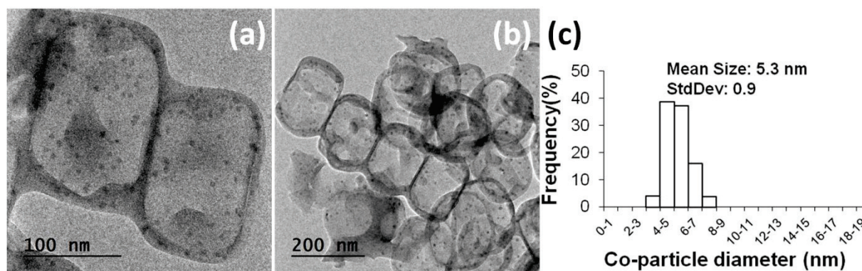
Figure 21: TEM images (a,b) and Co particle size distribution (c) of 3-Co@ZSM-5-DS, obtained by desilication with 0.6M Na_2CO_3 then reduced at 750°C for 3 hours.
