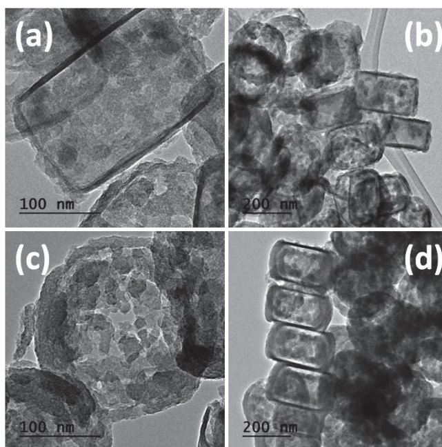
Figure 8: TEM images of hollow ZSM-5 obtained by treating parent ZSM-5 with different Si/Al, 280 (a and b) and 493 (c and d) with 0.6 M \text{Na}_2\text{CO}_3 solution at 80°C for 12 hours.
