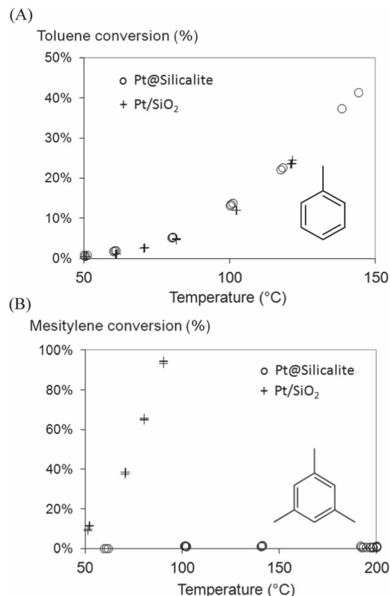
Fig. 3 Conversion during the hydrogenation of (A) toluene and (B) mesitylene over the Pt@silicalite-1 and a Pt/SiO 2 . Toluene pressure = 903 Pa, balance H 2 . Mesitylene pressure = 61 Pa, balance H 2 .
