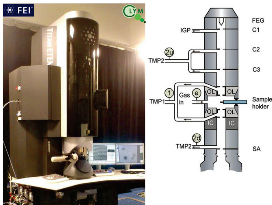
Figure 2: The photo (left) and sketch of the vacuum system(right) of the ETEM apparatus. vacuum system highlighting the pressure-limiting apertures at the stages of the objective lens (OL), the condenser lenses (first (C1), second (C2) and third (C3)) and the selected area (SA) aperture. 6
