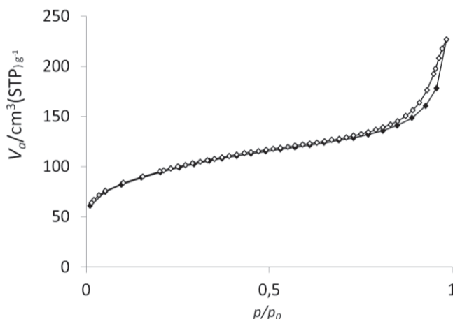
Figure 9 : N_2 adsorption/desorption isotherms of hollow ZSM-5 obtained by treating parent ZSM-5 with Si/Al=280 with 0.6M Na_2CO_3 at 80°C for 12hours.
