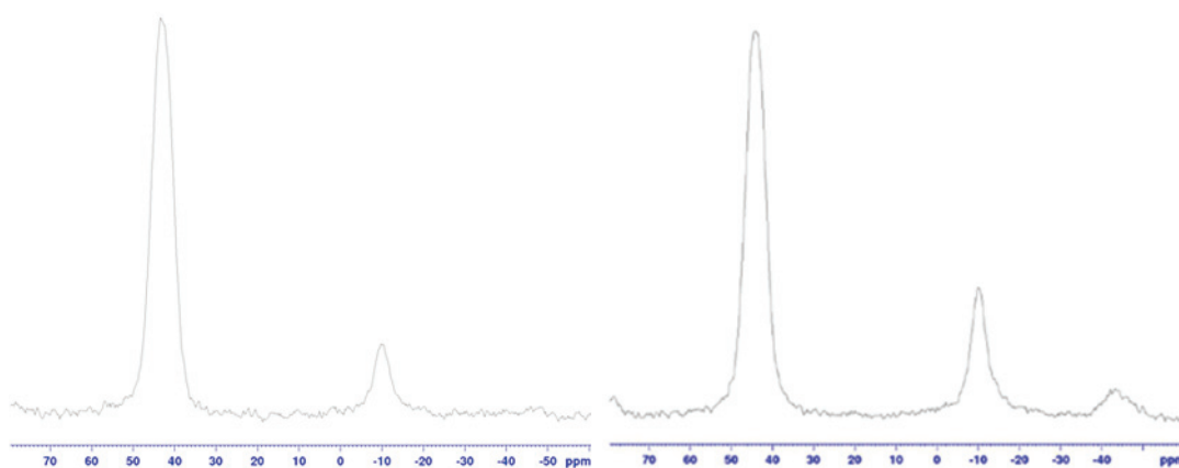
Figure 15: ^{27}\text{Al} NMR spectra of hollow ZSM-5 before (left) and after (right) calcination.
