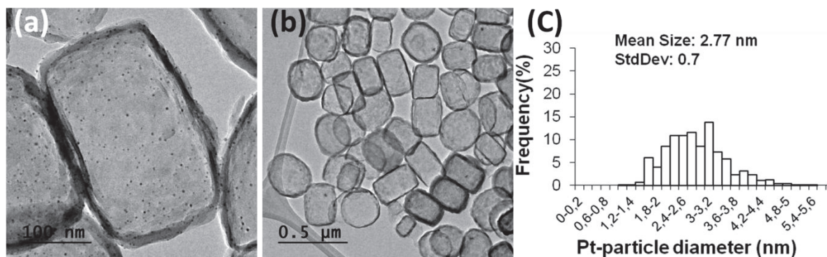
Figure 23: TEM images (a,b) and Pt particle size distribution (c) of 1.5-Pt@ZSM-5-DS reduced in \text{H}_2 at 750°C for 3 hours.
