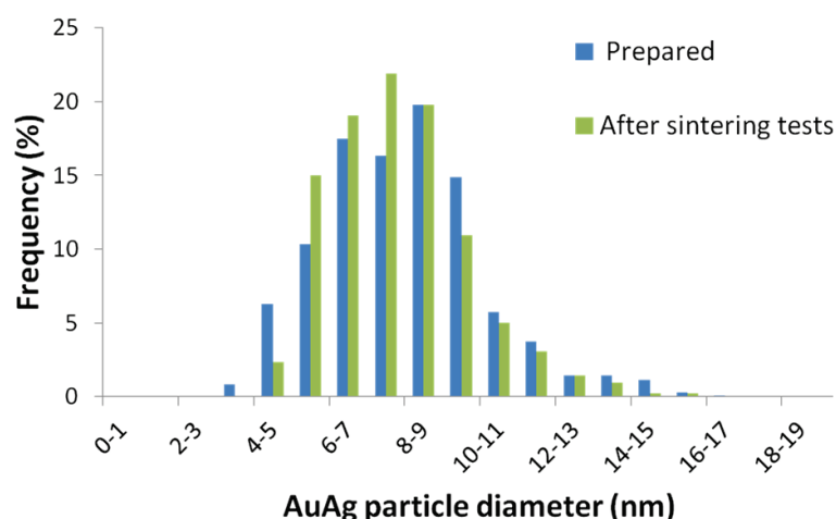
Figure 26: Particle size distribution of \text{Au}_{0.53}\text{Ag}_{0.04}\text{@Sil-1} before (■) and after sintering test (■).
