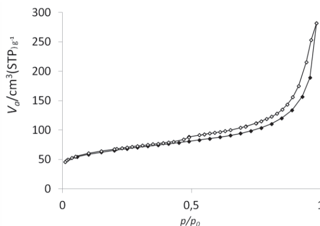
Figure 20 : N_2 adsorption/desorption isotherms of Co@ZSM-5-DS obtained by desilication with 0.6M Na_2CO_3 then reduced at 750°C for 3 hours.
