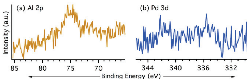
Figure 18: XPS spectra Al 2p (a) and Pd 3d (b) of \text{Pt}_{0.27}\text{Pd}_{0.17}\text{@ZSM-5-DR} sample.
