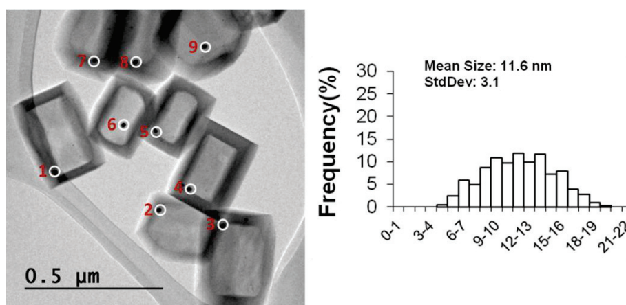
Figure 16: TEM image (left) and particle size distribution (right) of \text{Pt}_{0.27}\text{Pd}_{0.17}\text{@ZSM-5-DR} sample. White circles indicate the areas for EDX detection with corresponding spot numbers on the left. Only one of the biggest particle in each shell are counted for the particle size distribution (several small particles with diameter about 2 nm are co-existed in the shell of ZSM-5 which will show in Fig. 17 and will be discussed in the following paragraphs).
