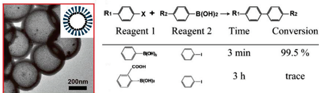
Figure 12: TEM image of \text{Pd@mesoporous SiO}_2 (left); Suzuki Reaction of phenylboronic Acid, o-carboxyphenylboronic acid and iodobenzene catalyzed by \text{Pd@meso-SiO}_2 (right). Reaction conditions: 80 °C, ethanol (10 mL), iodobenzene (0.5 mmol), phenylboronic acid (1 mmol), \text{K}_2\text{CO}_3 (1 mmol), and catalyst (10 mg), (from ref 116 ).
