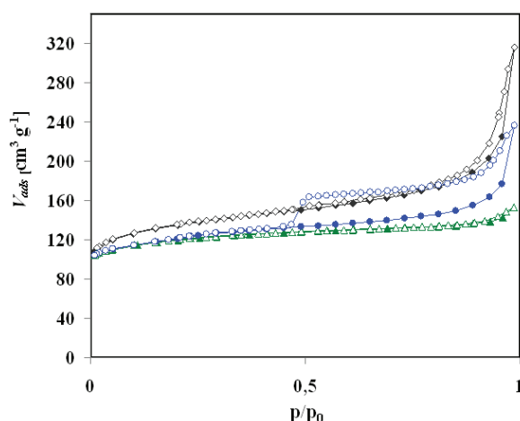
Figure 26: \text{N}_2 adsorption/desorption isotherms of (top-down order) 1.5-Pt@ZSM-5-DS (◆), 1.02-Pt@ZSM-5-DR (●) and 0.98-Pt/ZSM-5 (▲).
