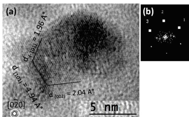
Figure 18: HRTEM picture (a) and corresponding Fast Fourier Transform (FFT) diffraction patterns (b) of a cobalt particle from 18.5-Co@ZSM-5-DS treated by 0.6M \text{Na}_2\text{CO}_3 reduced at 750°C for 3 hours sample.
