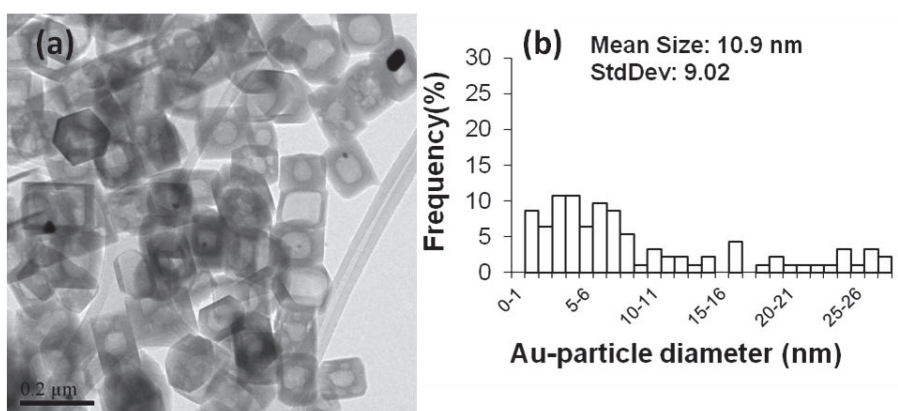
Figure 1: TEM image (a) and particle size distribution (b) of Au@Sil-1-PI sample.
