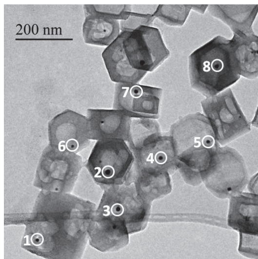
Figure 29: TEM image of \text{Au}_{0.53}\text{Ag}_{0.04}@\text{Sil-1} after CO oxidation. White circles indicating the areas for EDX detecting with the corresponding spot number on the left.
