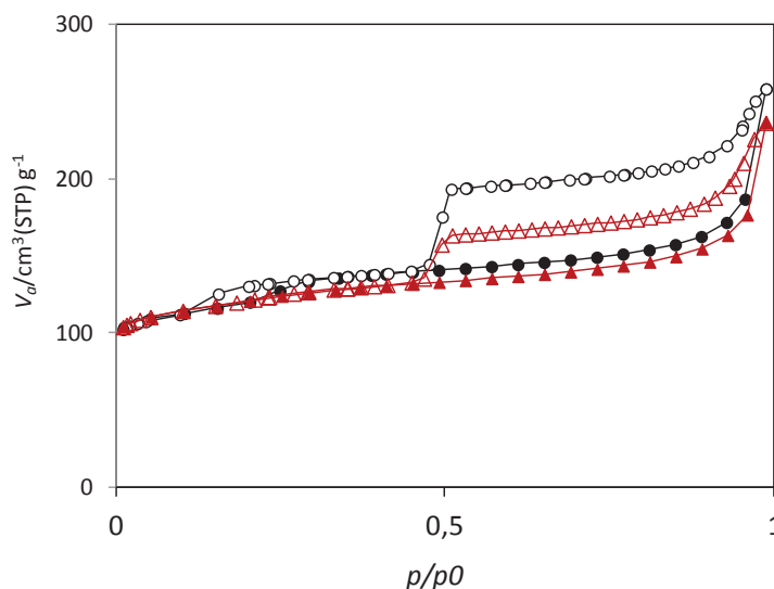
Figure 14: N_2 adsorption/desorption isotherms of hollow silicalite-1( \circ ) and hollow ZSM-5-DR ( \Delta ) at 77K.
