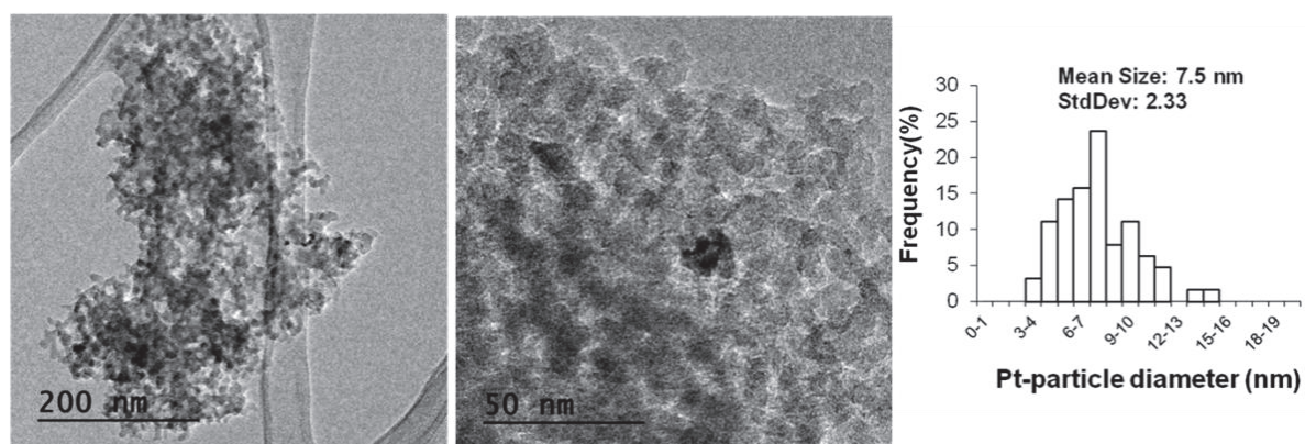
Figure 27: TEM images and particle size distribution of Pt/SiO 2 -C catalyst.
