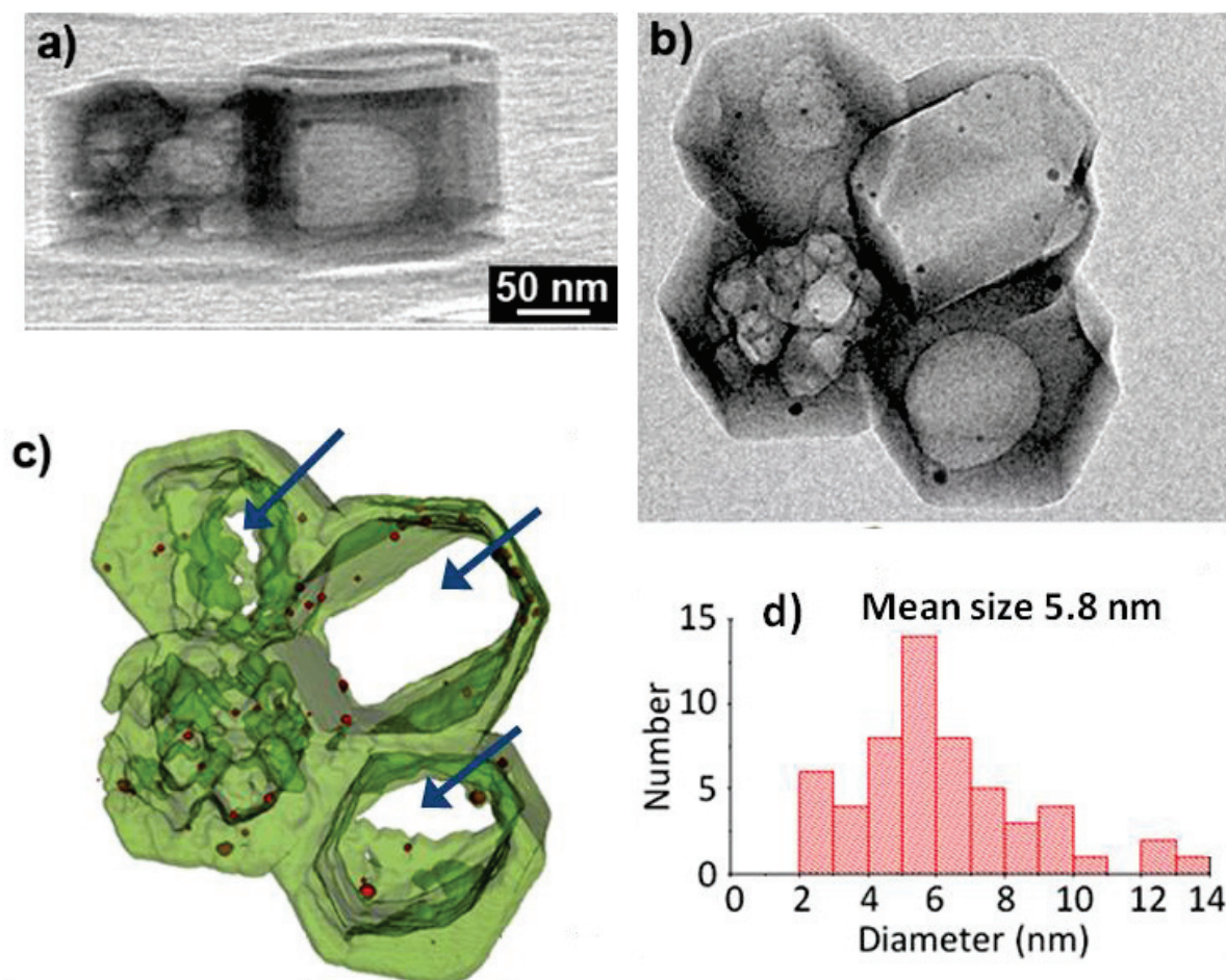
Figure 15: Video frames of fast single-tilt tomography on 1-Ag@Sil-1 (a, b) (the limits of a continuous tilting series acquired in bright field in less than 4 minutes from 78° to -38.5° under high vacuum at 20°C and 300 kV); surface rendering obtained by reconstruction from the tomography video (c) and size histogram of Ag NPs (d).
