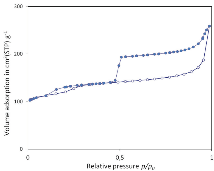
Figure 11: N 2 adsorption/desorption isotherms of 0.9-Pt@Sil-1 sample.
