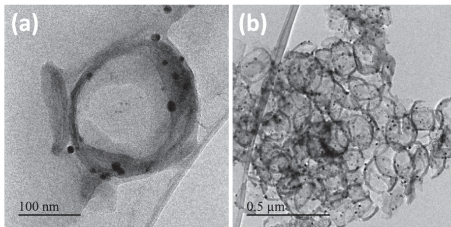
Figure 22: TEM pictures of 21-Ni@ZSM-5-DS, obtained by desilication with 1 M \text{Na}_2\text{CO}_3 then reduced at 750°C for 3 hours.
