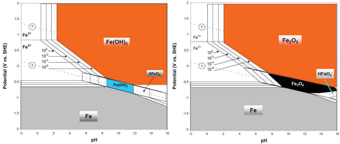
Figure 2Left: E-pH diagram of iron or steel with four concentrations of soluble species, three soluble species and two wet corrosion products (25°C). Right: E-pH diagram of iron or steel with four concentrations of soluble species, three soluble species and two dry corrosion products (25°C)
