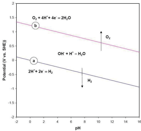
E-pH stability diagram of water at 25°C
