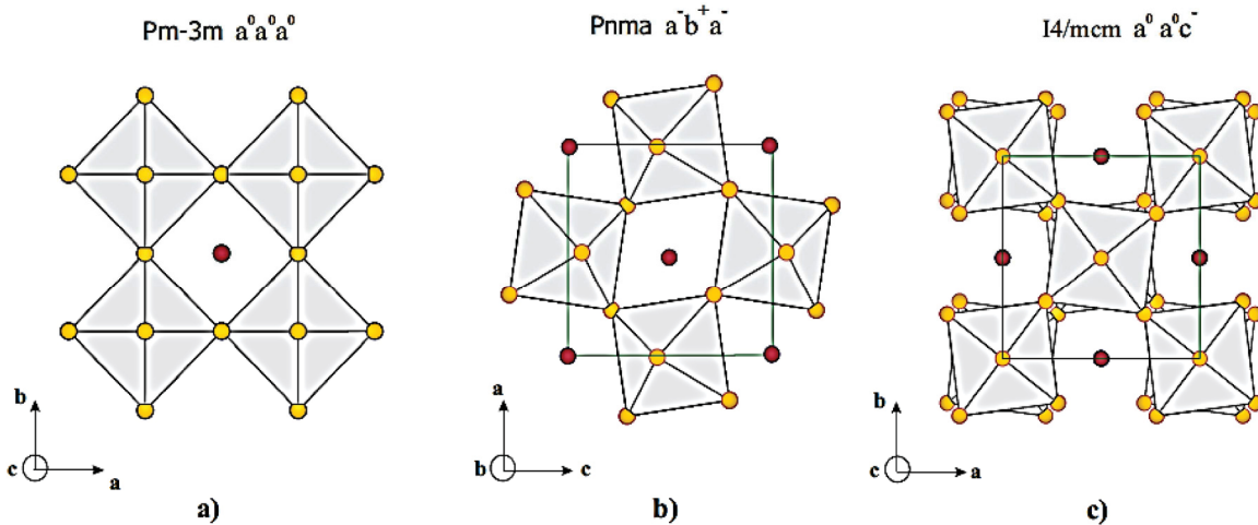
Figure 2: Glazers notation and tilting/distortions for (a) cubic, (b) orthorhombic and (c) tetragonal structure [From Thesis of Cecile Autret, CRISMAT].
