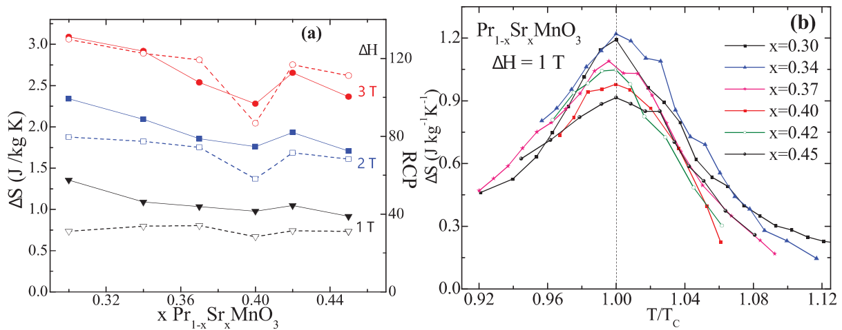
Figure 19: (a) Entropy change (solid symbol) their corresponding RCP (open symbol) for all samples. (b) Entropy change for field change of 1 T for all samples, temperature is normalized with their T_c .
