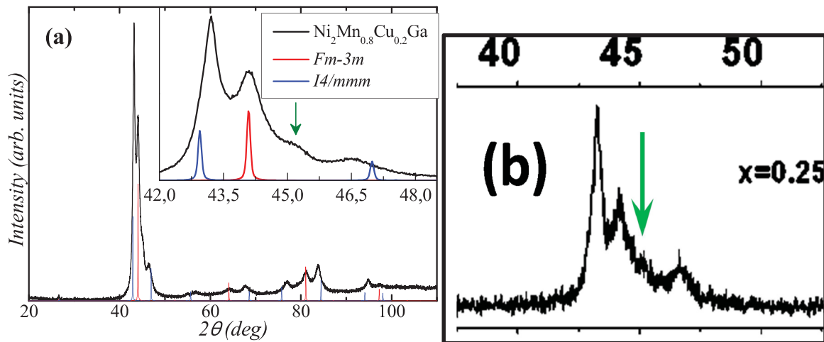
Figure 8: XRD pattern for Ni 2 Mn 0.8 Cu 0.2 Ga (a) Comparison of experimental spectra with calculated spectra of cubic Fm-3m and tetragonal I4/mmm . Inset display peaks between 2θ= 42° & 48°. Expand view around intense peak (2θ=45°) of Ni 2 Mn 1-x Cu x Ga data from [30]) demonstrating extra peak (green arrow) for x=0.25.
