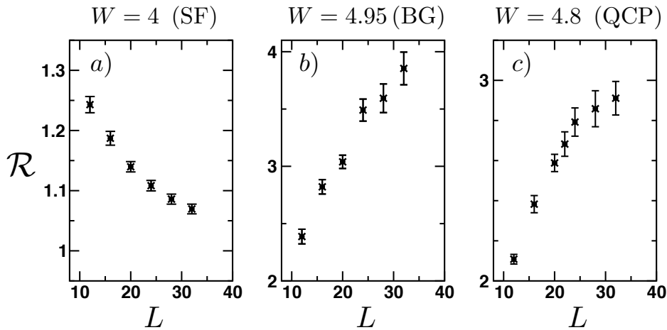
Figure IV.17: Evolution of \mathcal{R} = \rho_{\text{sf}}^{\text{avg}} / \rho_{\text{sf}}^{\text{typ}} with system size L inside the different phases and at criticality. Panel a: In the SF phase W = 4 , \mathcal{R} tends to 1 for increasing system size L , signalling a self-averaging SF phase. Panel b: Inside the BG phase ( W = 4.95 ) \mathcal{R} increases with system size indicating a lack of self-averaging. Panel c: At criticality, the ratio \mathcal{R} seems to saturate for big system sizes to a finite value > 1 , i.e. the critical point is not self-averaging but has different nature than the BG phase.
