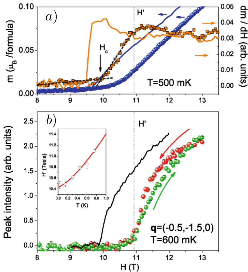
Figure I.5: Panel a): Field dependence of magnetization (Boson density), in blue, and susceptibility (compressibility of the Bose gas), in orange, as measured in the clean (CH_3)_2CHNH_3CuCl_3 (solid lines) and the doped (CH_3)_2CHNH_3Cu(Cl_{1-x}Br_x)_3 , x = 0.05 (symbols) magnetic insulators. Panel b) Field dependencies of intensity of the antiferromagnetic Bragg peaks (square of the BEC order parameter) in the two respective materials. Data obtained in Ref. [140]. The figure is taken from Ref. [114].
