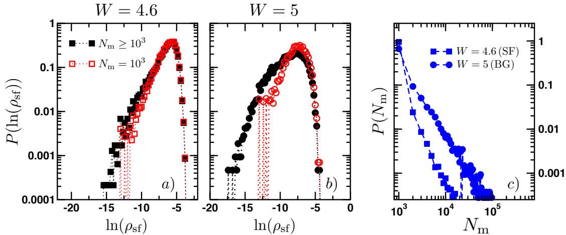
Figure IV.12: a) Distribution of \ln(\rho_{\text{sf}}) for a system of size N = 24 \times 24 at disorder strength W = 4.6 (SF phase) with 1000 measurement steps (red) and with the dynamical adjustment of the measurement steps (black). b) Distribution of the same quantity for the same size inside the Bose glass phase ( W = 5 ). The dynamical adjustment procedure allows for the measurement of much smaller superfluid densities, specially inside the Bose glass phase. c) Distribution of the number of Monte Carlo measurement steps N_m needed for the two disorder strengths in panels a) and b) . In the superfluid phase only 10% of the disordered samples required more than 10^3 measurement steps, this goes up to around 30% inside the Bose glass phase.
