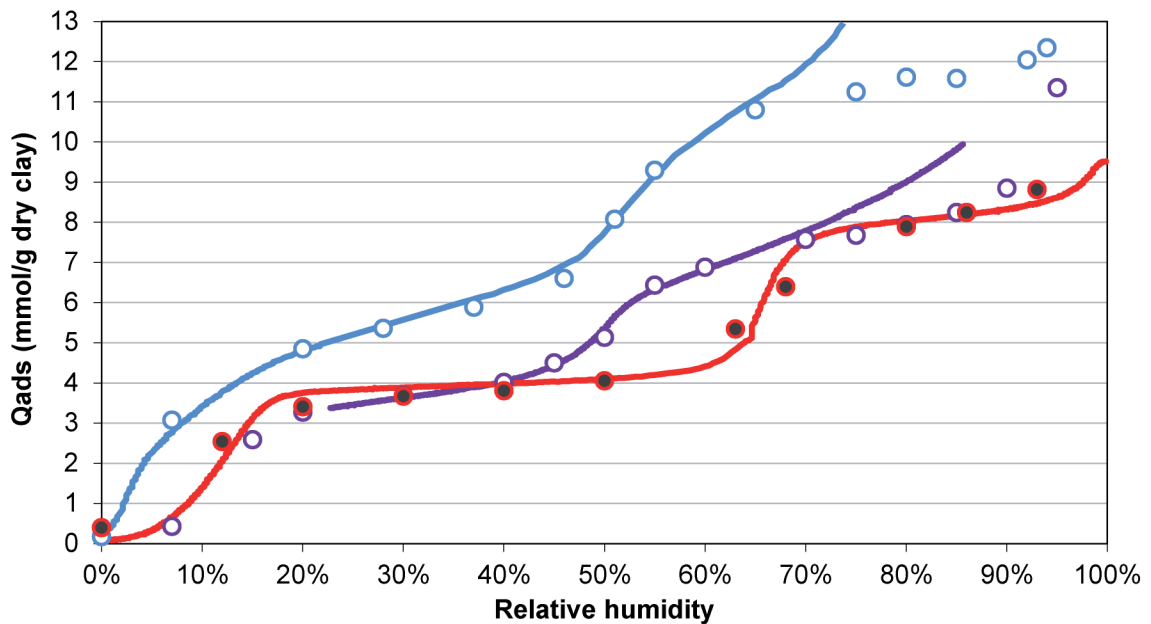
Figure 6-1 Smectite water content ( Q_{ads} ) as a function of relative humidity. Solid lines were obtained from water vapor desorption isotherms, whereas dots represent \text{H}_2\text{O} contents used for XRD profile modeling. Blue, purple, and red patterns represent OH-Hydr, F-Hydr, and F-HT samples, respectively.
