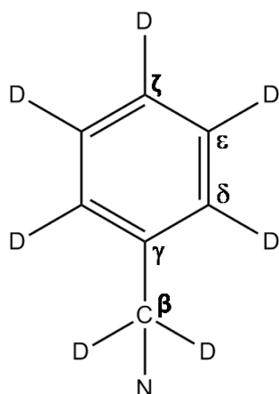
Figure 32: Schematic drawing of the [\text{d}_7] -benzyl.
