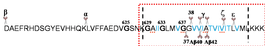
Figure 2: Partial sequence of the APP where the TM domain is enclosed by dashed lines. The red rectangle marks the region synthesized for this study. Underlined are isotopically-labeled amino acids that were incorporated for solid-state nuclear magnetic resonance (ss-NMR) studies. The \beta -branched amino acids are marked in blue. The positions of the glycines in the 3 consecutive GxxxG are presented in bold and labeled. The cleavage sites of \alpha -, \beta -, \gamma -secretase are indicated with scissors.
