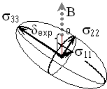
Figure 6: Graphical representation of the chemical shift anisotropy (CSA) tensor (cf. text). The length of the principal axes of the tensor is represented by 1/\sigma_{ii} , with \sigma_{ii} being the main tensor elements \sigma_{11} , \sigma_{22} , \sigma_{33} [Bechinger and Sizon, 2003].
