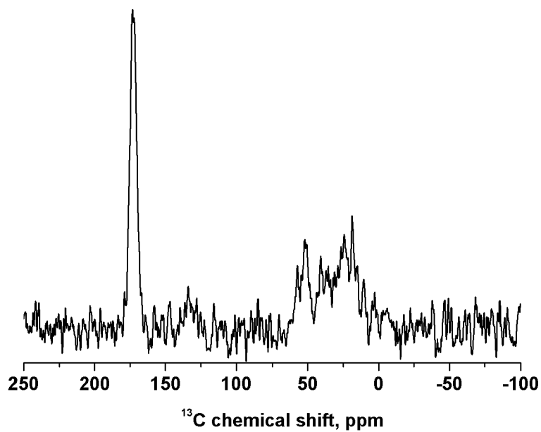
(a) ^{13}\text{C} chemical shifts from Glu22 of \text{A}\beta(1-40) , natural abundance and MOPS molecules. Collected at 294 K.
