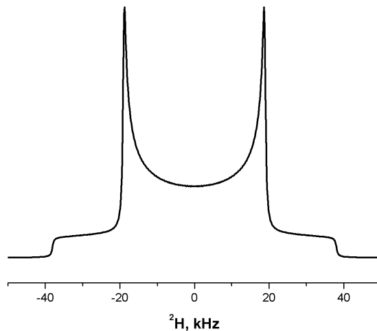
Figure 11: ^2\text{H} powder pattern spectrum arising from two transitions, eq. 2.4.
