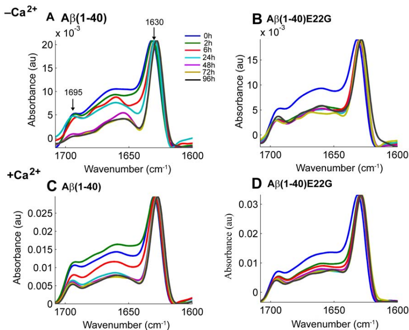
Figure 3. ATR-FTIR spectra of A \beta (1–40) and A \beta (1–40)E22G. FTIR spectra of A \beta (1–40) and A \beta (1–40)E22G were taken in the presence and in the absence of added Ca 2+ , showing the amide I region of the spectra (1600–1700 cm -1 ). Aliquots of 2 \mu l were taken from each sample at t=0, 2, 6, 24, 48, 72, and 96 h (shown in blue, green, red, cyan, purple, mustard, and dark blue, respectively). The data shown here were collected in one continuous experiment and are representative of three independent trials. doi:10.1371/journal.pone.0018250.g003
