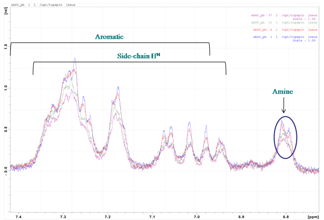
Figure 54: NMR spectrum of A \beta (1-40) in phosphate buffer. (a) full spectrum, (b) closeup into the aromatic and amine regions.
