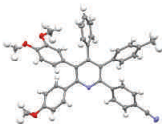
Figure 1 ORTEP drawing of 36 with 50% probability displacement ellipsoids
