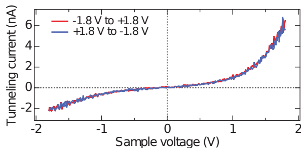
Figure 14.5. – Current-voltage curve acquired atop the center of a single Fe-phen HS molecule on Cu(100) . The spectrum exhibits a normal tunneling background with no sign of a spin transition. The feedback loop is opened at 1.8 V and 6 nA.
