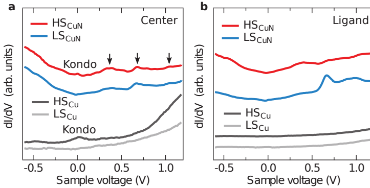
Figure 14.9. – dI/dV spectra on Fe-phen molecules for both spin states on CuN/Cu(100) and Cu(100) . a , dI/dV spectra taken on top of Fe-phen molecules' center. The Kondo resonance is distinguishable for molecules in the HS state on both substrates. The arrows indicate the position of additional spectroscopic features that are observed when the molecules are on the CuN/Cu(100) surface (peaks located at 0.35, 0.7 and 1.0 eV). b , dI/dV spectra acquired on the top of the ligand of Fe-phen molecules on CuN/Cu(100) and Cu(100) surfaces. The spectra were acquired with a voltage modulation of 10 mV at a frequency of 723 Hz.
