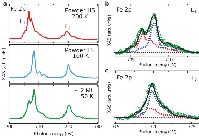
Figure 14.3. – Coexistence of HS and LS states of Fe-phen molecules on Cu(100) revealed by XAS. a , XAS performed at the Fe L edges on Fe-phen powder reference sample at 200 K (HS state, top panel), at 100 K (LS state, middle panel) and on 2 ML Fe-phen on Cu(100) at 50 K (bottom panel). The main peak of the L_3 edge is located at different energies for the HS (top) and the LS (middle) Fe-phen molecules. The 2 ML-thin Fe-phen film (bottom) seems to have HS and LS contributions. Reproduction of the XAS (solid black) b , L_3 and c , L_2 edges of 2 ML Fe-phen on Cu(100) (green circles) using a linear combination of the HS (46%, red) and the LS (54%, blue) reference spectra obtained on the powder sample.
