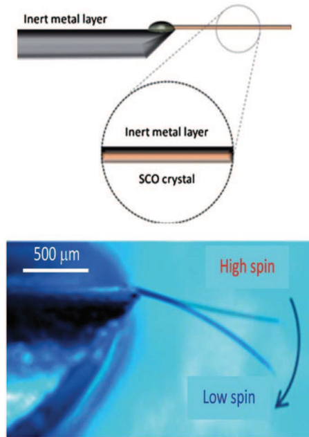
Figure 12.16. – SCO-based cantilever prototype. (Top) Bilayer strip composed of a thin film of aluminum and the SCO complex \text{Fe}(\text{3-CNpyridine})[\text{Au}(\text{CN})_2]_2 \cdot 2/3\text{H}_2\text{O} . (Bottom) Highlight of the SCO-induced actuation of the bilayer cantilever by optical microscopy image. The figure is taken from Ref. 351.
