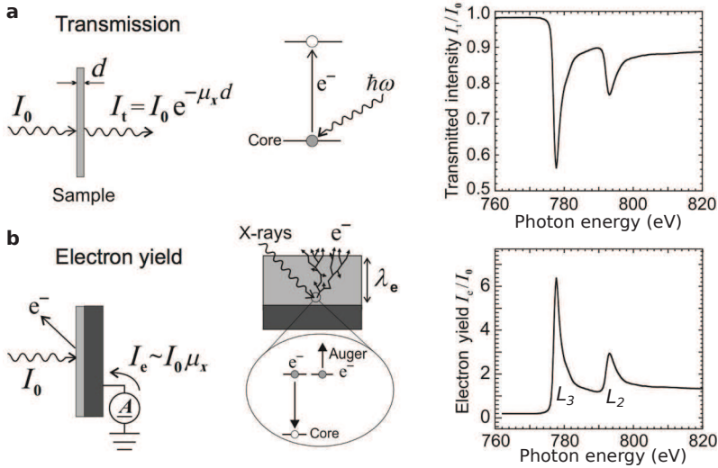
Figure 4.2. – Two different common techniques for measuring X-ray absorption. a , (Left) Typical transmission geometry where the proportion of X-rays that goes through the sample is measured. (Center) Schematic of a photon-induced core-level electron excitation that corresponds to an absorption event. (Right) Transmitted intensity as a function of the photon energy for a 10 nm Co-film sample. b , Experimental principle and methods to measure X-ray absorption spectra by (total) electron yield detection. (Left) Experimental geometry for total electron yield detection: the X-rays irradiate the sample and a picoammeter measure the current that goes from the sample to the ground. (Center) The absorption of photons induces core holes that may lead to Auger-electron emission. The inelastic scattering of primary Auger electrons produce a cascade of secondary electrons through inelastic scattering. A proportion of the Auger and secondary electrons escape from the surface; and electrons are flowing from the ground to the sample to keep charge neutrality. The total number of emitted electrons is proportional to the number of Auger electrons, that in turn is proportional to the absorption cross section. (Right) Electron yield intensity as a function of the photon energy for a Co sample. The X-ray absorption spectrum show two distinct peaks that correspond to the L_3 edge (transition from a 2p_{3/2} state) and the L_2 edge (transition from a 2p_{1/2} state). The figure is adapted from Ref. 84.
