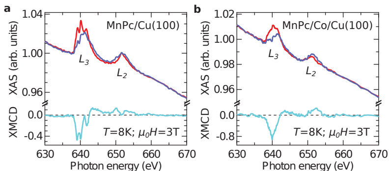
Figure 8.7. – XAS and XMCD spectra at the Mn L_{3,2} edges for MnPc on Cu(100) and Co/Cu(100) substrates. XAS and the corresponding normalized XMCD spectra at the Mn L_{3,2} edges for a , 1 ML MnPc on Cu(100) and b , 0.5 ML MnPc on Co/Cu(100). The spectra were acquired at T = 8 K under an external magnetic field \mu_0 H = 3 T. The magnetic field is applied along the incoming direction of the photon, which makes an angle of 30^\circ with the surface plane.
