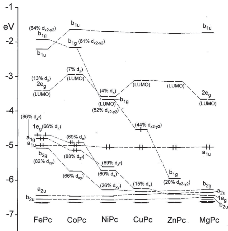
Figure 8.3. – Calculated orbital energy levels of different MPc molecules. The orbitals are labeled according to the irreducible representation D_{4h} (see text). The population of some orbitals are indicated in parentheses. The figure is taken from Ref. 203.
