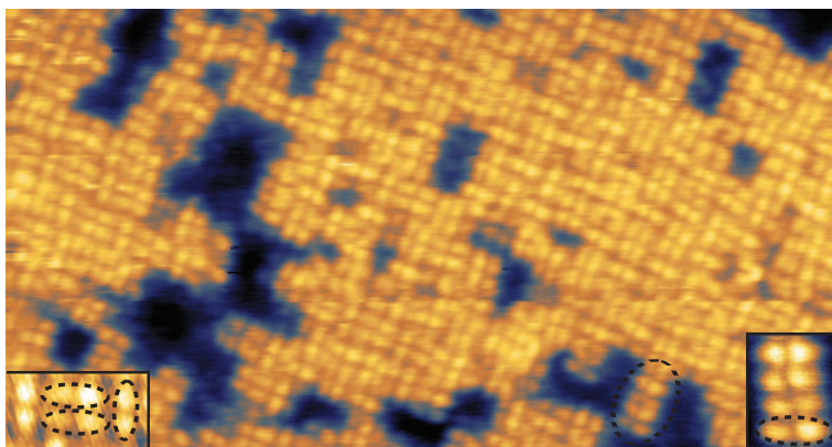
Figure 13.5. – Molecular structure of the second-ML Fe-phen molecules on Cu(100). STM topography of the second-ML Fe-phen molecules on Cu(100) revealing dense and depleted areas of molecules. The bottom left inset shows the three-molecule pattern commonly seen in the dense and ordered areas. Other molecular structures seldom appear, such as the one presented in the bottom right inset: molecules with same orientation are sitting next to each other, so as to form a chain-like molecular structure. Image size is 27.6 \text{ nm} \times 14.5 \text{ nm} ( V=0.6 \text{ V}, I=115 \text{ pA} ). Inset sizes are (left) 2.8 \text{ nm} \times 1.6 \text{ nm} , (right) 1.6 \text{ nm} \times 2.1 \text{ nm} .
