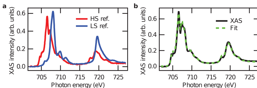
Figure 12.11. – XAS on the Fe L edge of Fe-phen powder. a , LS and HS reference spectra acquired at 100 and 300 K, respectively. b , XAS spectrum acquired at 30 K where a proportion of molecules are in the metastable HS state due to the X-rays. The experimental spectrum can be reproduced by a linear combination of the LS and HS reference spectra (22% LS and 78% HS) that allows to extract the proportion of HS molecules: 78%. See Refs. 280, 333 for more details.
