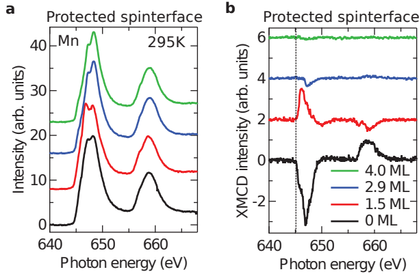
Figure 10.3. – XAS and XMCD at the Mn L_{3,2} edges of MnPc on Cu( d_{Cu} )/Co(100) for different Cu thicknesses. a , White line spectra at the Mn L_{3,2} edges of MnPc on Cu( d_{Cu} )/Co(100) for d_{Cu} = 0 ML, 1.5 ML, 2.9 ML and 4.0 ML. b , XMCD spectra at the Mn L_{3,2} edges of MnPc on Cu( d_{Cu} )/Co(100) for the Cu thicknesses enumerated in a . The spectra were acquired at 295 K in 0.1 T, and are vertically shifted for clarity.
