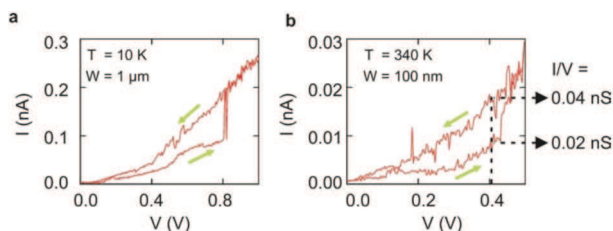
Figure 12.13. – I-V characteristics on a single nanoparticle. a , Current-voltage curve acquired at low temperature ( T = 10 K) on Fe-based SCO nanoparticles bridged between two 1\ \mu\text{m} -width gold electrodes. b , Same measurements performed at T = 340 K on a single nanoparticle sandwiched between two 100\ \text{nm} -width gold electrodes. In both panels, we observe a conductance jump ascribed by the authors to a transition from the LS to the HS state when increasing the voltage. The figure is taken from Ref. 341.
