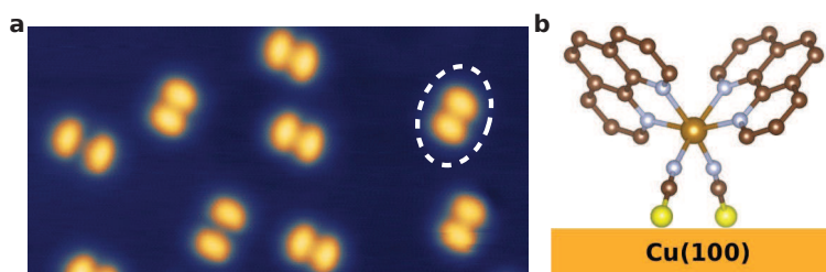
Figure 13.1. – Isolated molecules on Cu(100). a , Topography of single Fe-phen on Cu(100). A single Fe-phen molecule appears as two bright lobes corresponding to its two phenanthroline groups. A single molecule is encircled for clarity. Image size is 17\text{ nm} \times 8.5\text{ nm} ( V=30\text{ mV}, I=2\text{ nA} ). b , Model of a single Fe-phen on top of Cu schematizing the adsorption geometry of the single molecules.
