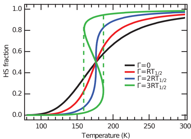
Figure 12.3. – Proportion of high-spin molecule as a function of temperature. The different temperature-dependent proportions of HS molecules were calculated using Eq. 12.6 considering different values for the cooperative term \Gamma . We used \Delta H = 8600 \text{ J mol}^{-1} and \Delta S = 48.78 \text{ J mol}^{-1} \text{ K}^{-1} corresponding to the enthalpy and entropy variation of Fe-phen. 277
