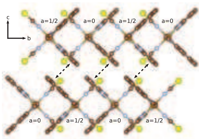
Figure 12.2. – Bulk structure of Fe-phen. The unit cell contains four molecules and is repeated once along the b axis. The figure has been created with VESTA 273 using the crystallographic data from Gallois et al. 266
