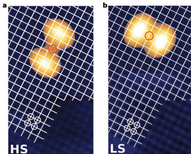
Figure 15.4. – Adsorption site of first-ML Fe-phen on Cu(100). Topographies of single a , HS Fe-phen and b , LS Fe-phen molecules atop an atomically resolved Cu(100) surface revealing the adsorption site of the molecule. The Fe ion of the HS and LS molecules is sitting on top of a hollow and bridge sites, respectively. For clarity, four Cu atoms are encircled and intersections of lines represent the center of Cu atoms. Image sizes are 2.8 \text{ nm} \times 5.0 \text{ nm} .
