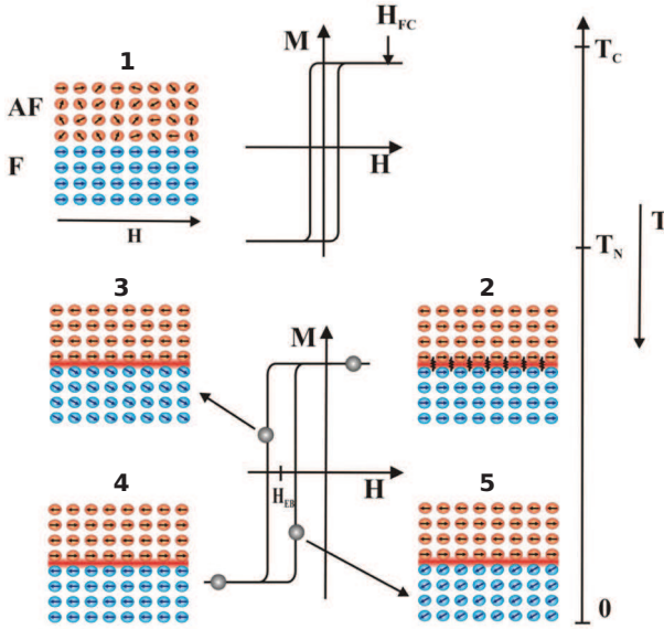
Figure 3.1. – Phenomenological picture of exchange bias for an AF-FM bilayer. Step 1 for T_N < T < T_C , the FM layer is magnetically ordered while the AF layer is disordered. The corresponding hysteresis loop resembles that of a normal FM layer with the magnetic field H aligned along the easy axis of the FM layer. Step 2 shows the magnetic state of the bilayer after cooling below T_N in a positive external magnetic field. Both AF and FM layers are magnetically ordered and both layers are magnetically coupled between them. The negative magnetic field to apply for rotating the magnetic moments of the FM layer is relatively large due to the interactions with the AF layer, as represented in step 3. Step 4, the magnetic moments of the FM layer can be fully reversed while the magnetic moments of the AF layer stay similar to that of step 2 and 3. In step 5, the magnetization reversal of the FM layer can occur for a negative external field as the AF-FM interactions favor the magnetic configuration of step 2. The resulting hysteresis curve for T < T_N is shifted by H_{EB} due to exchange bias. The figure is taken from Ref. 16.
