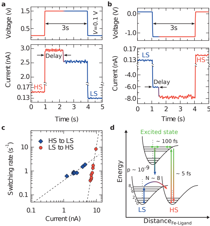
Figure 14.12. – Proposed mechanism for the spin-state switching of Fe-phen on CuN/Cu(100). a, (b) Real-time voltage and current traces of a voltage-pulse induced HS to LS (LS to HS) transition. The voltage pulse of 1.5 V (–1.2 V) is applied for 3 s and the spin-state of the Fe-phen molecule is read from the tunneling current at a voltage of 0.1 V. The HS to LS (LS to HS) transition is witnessed during the pulse by a small decrease (increase) of the current after a delay of 1.3 s (0.4 s). c , Observed switching rate (defined as one over the switching delay) as a function of the tunneling current during the voltage pulse. The tip is initially stabilized at 0.1 V and 100 pA and the different currents are obtained by slightly varying the intensity of the voltage pulse. The dashed lines indicate the results of power-law fits of the switching rate as a function of the current. d , Schematic of the proposed spin-state-switching mechanism in both directions. While, the switching from the HS to the LS state is a one electron process ( N \approx 1 ) and involves an excited state, the reverse switching (from LS to HS) is a higher order process ( N = 8 ) that can involve the population of intermediate vibrational levels (heating).
