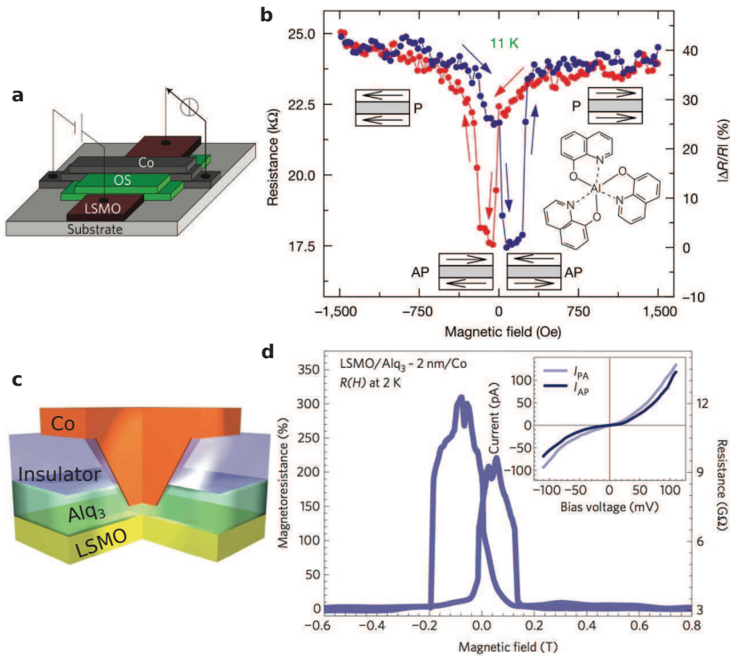
Figure 7.4. – Magnetoconductance in Alq 3 -based organic spin valves. a , Schematic of a typical vertical organic spin-valve device. The OSC (here Alq 3 ) is sandwiched between a bottom LSMO and a top Co electrodes. Magnetoconductance measurements are performed by applying a bias voltage between the magnetic electrodes and measuring the current as a function of an external in-plane magnetic field. b , Magnetoconductance loop of a spin-valve device such as presented in a (LSMO(100 nm)/Alq 3 (130 nm)/Co(3.5 nm)) at 11 K. The lower resistance is obtained for an antiparallel magnetic alignment of the electrodes and the device is thus defined as an inverse spin valve. c , Schematic of an organic magnetic tunnel junction obtained by nanoindentation into the organic layer before deposition of the top Co electrode. d , Magnetoconductance measurements of an organic magnetic tunnel junction (see c ; LSMO/Alq 3 (2 nm)/Co) at 2 K and with a bias voltage of -5 mV. The lower resistance is here obtained for a parallel magnetic alignment of the electrodes, i.e. different from the device measured in b . The figure is adapted from Refs. 4, 171, 172.
