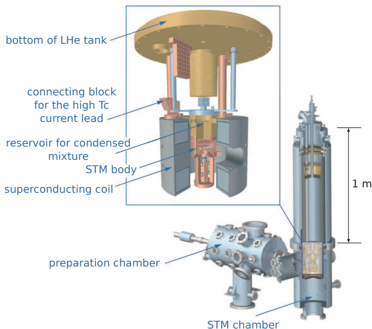
Figure 6.1. – Technical drawing of the Joule-Thomson STM. View of the STM and preparation chambers. The inset magnifies the reservoir for the condensed mixture on top of the STM stage. Note that the investigated surfaces are facing downwards. The figure is taken from Ref. 105 and a full description can be found in Ref. 125.
