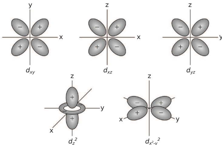
Figure 2.1. – The five different d atomic orbitals. The figure is adapted from Ref. 8.
