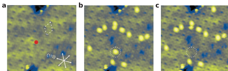
Figure 12.14. – STM topographies revealing spin transition of SCO complexes. a , Topography of a 14 nm wide area. The second-layer molecules appear in yellowish and are prepared in the LS state. The tip is afterward positioned on top of the red dot. b , Topography of the same location than a but recorded after a voltage pulse. The brighter molecules correspond to molecules switched into the HS state. Selective reverse switching can be performed by placing the tip on top of a HS molecule ( e.g. the encircled HS molecule) and increasing the tunneling current to 0.5 nA with a voltage of 1.8 V for about 0.5 s. The topography acquired afterwards is presented in c where the encircled molecule is now in the LS state. The figure is taken from Ref. 347.
