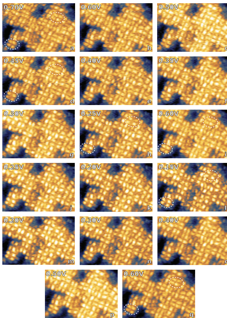
Figure C.1. – Voltage-dependence of the topography of second-ML Fe-phen on Cu(100). Different topographies of the same area are consecutively acquired with different sample voltages that are indicated on the images. Two pairs of second-ML Fe-phen molecules are encircled in some of the topographies. The sequence order goes from left to right; top to bottom. Image sizes are 9\text{ nm} \times 6\text{ nm} ( I=15\text{ pA} for the seven first images, and then I=1.4\text{ nA} ).
