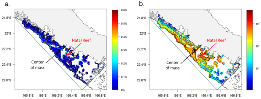
FIGURE 3.5 Maps of settlement using an 11-day precompetency period. For each simulation, the number of settlers was computed in square grid cells of 0.01^\circ in size. For each grid cell, the number of settlers was (a) averaged over the whole simulated period (1320 simulations) and presented as a percentage of the total number of larvae released and (b) calculated on a logarithmic scale as \log_{10}(N_i + 1) where N_i is the number of larvae settling in grid cell i .
