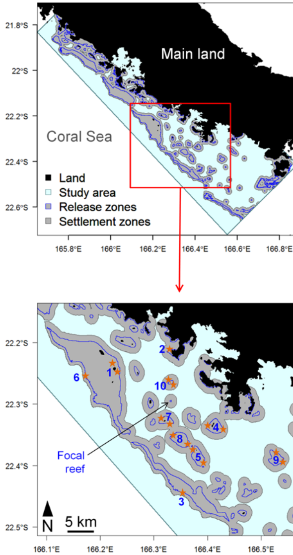
FIGURE 6.1 Study area : the South-West Lagoon of New Caledonia (SWL). The area in light blue represents the delimitation of the biophysical model. Release zones are delimited in blue. Settlement zones are depicted in grey and correspond to release zones buffered by a 1-km sensory zone. Land is shown in black. Localization of the focal reef and the 10 neighboring reefs (numbered from 1 to 10) is shown with orange stars indicating juveniles sampling stations on the 10 neighboring reefs.
