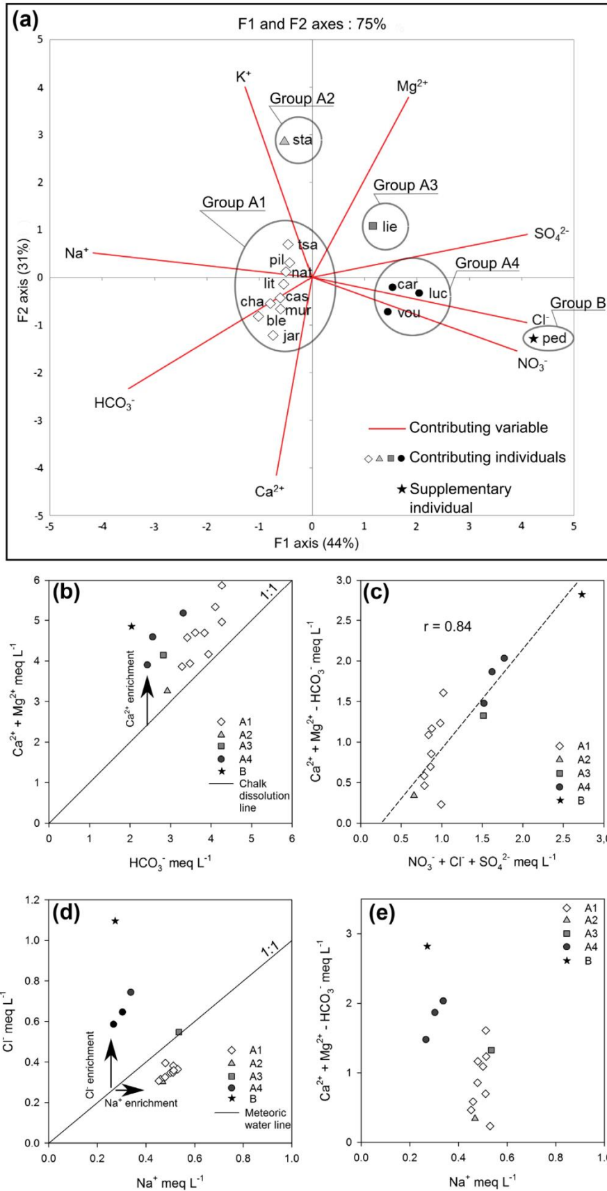
Fig. 5. (a) PCA of the groundwater geochemistry (14 contributing individuals: cas, cha, ble, pil, jar, lit, mur, nat, tsa, sta, lie, luc, vou, car; 1 supplementary individual: ped; 8 contributing variables: \text{HCO}_3^- , \text{Ca}^{2+} , \text{Mg}^{2+} , \text{Na}^+ , \text{Cl}^- , \text{K}^+ , \text{SO}_4^{2-} , \text{NO}_3^- ). Lakes are divided into 5 groups (A1: white diamond; A2: light-grey triangle; A3: dark-grey square; A4: black circle; and B: black star). (b) [\text{Ca}^{2+} + \text{Mg}^{2+}] versus \text{HCO}_3^- (solid line 1:1 represents the Chalk dissolution line). (c) [\text{Ca}^{2+} + \text{Mg}^{2+} - \text{HCO}_3^-] versus [\text{NO}_3^- + \text{Cl}^- + \text{SO}_4^{2-}] . (d) \text{Cl}^- versus \text{Na}^+ (solid line 1:1 represents the meteoric water line). (e) [\text{Ca}^{2+} + \text{Mg}^{2+} - \text{HCO}_3^-] versus \text{Na}^+ . Ion concentrations in meq L -1 .
