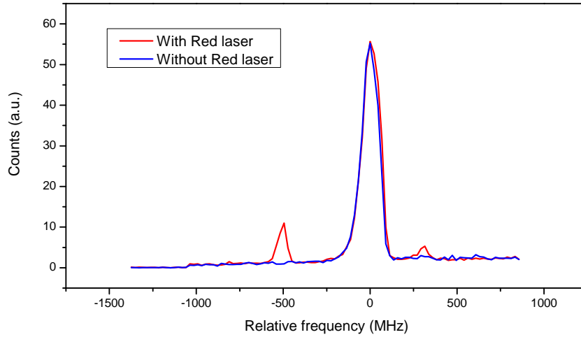
Figure III.8: One and two-photon transition lines for atoms trapped in a U-MOT at 600 \mu\text{m} from the chip surface. The red line corresponds to the case in which the 780 nm spectroscopic laser is on while the MOT is on. We can observe the two-photon transition line to the |60S_{1/2}\rangle Rydberg level on the left side of the spectra. The blue line shows the same signal when the 780 nm laser remains off during the data acquisition. We only observe then the nearly resonant stepwise excitation.
