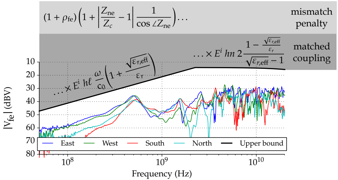
Figure 5.3: Upper bound versus measurement of an either-end mismatched ( 0 - 270 \Omega ), three-segment trace, after Figure 2.54c.
