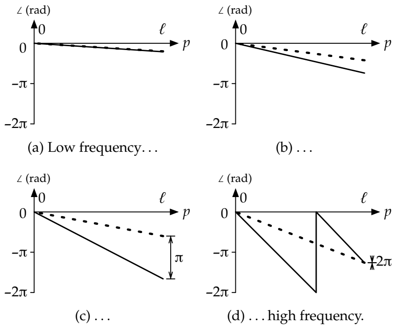
Figure 2.17: Phase along the transmission line of the line’s eigenwave \ell w (solid line) and illuminating plane wave \ell i (dashed line), for increasing frequency.
