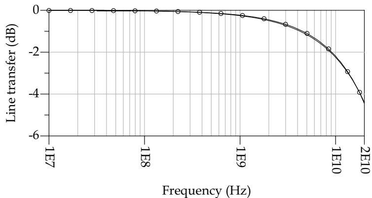
(c) Comparison of the rg loss model (curve with \circ markers) with ADS' MSUB model (plain curve) for the 5-cm case study microstrip.
