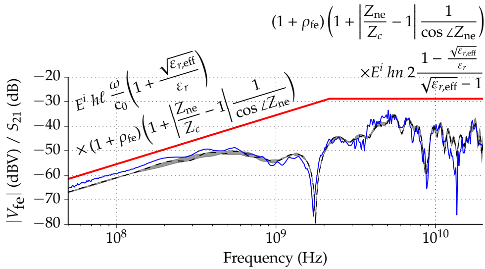
Figure 2.52: Measurement versus modified Taylor prediction of the coupling to a three-segment microstrip, shorted at the near end, matched at the far end. Port 1 is the GTEM cell input, port 2 is the trace’s far end.
