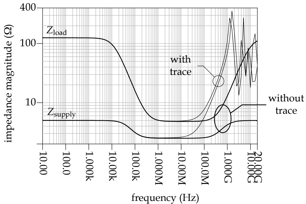
Figure 3.23: Impedance of specified source and load (thick curves) and the same impedances in series with 5 cm of 50 Ω trace (thin curves).
