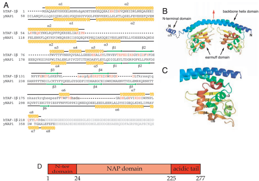
Figure 20: Structure of SET/TAF-Iβ/INHATΔC. 46
