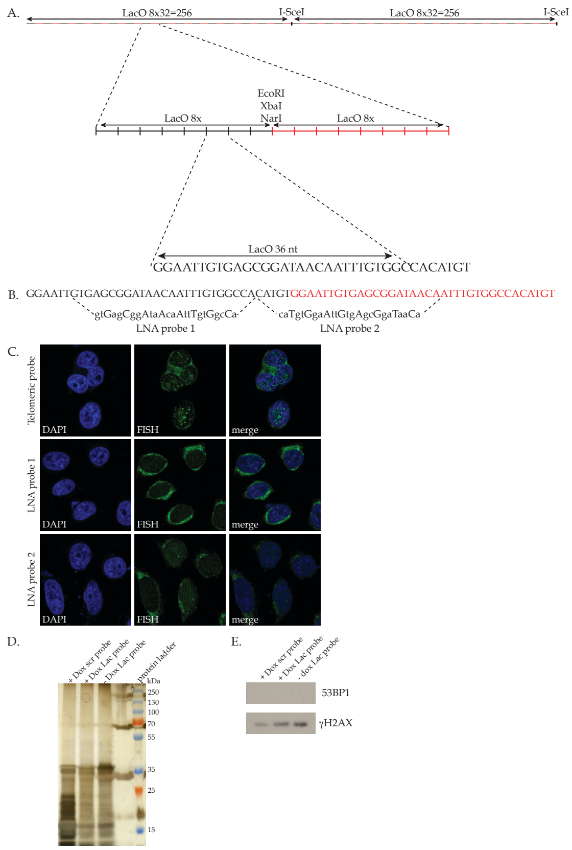
Figure 3: LacO-I-SceI array, LNA probes and PICh.
