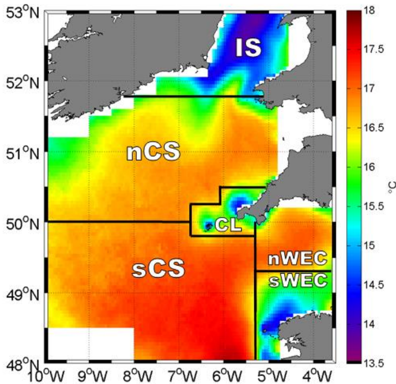
Figure 25: Mean July and August satellite SST ( ^{\circ}\text{C} ) between 2003 and 2013 with delimitation of defined hydrographical provinces: Irish Sea (IS), northern Celtic Sea (nCS), southern CS (sCS), Cap Lizard province (CL), northern Western English Channel (nWEC) and southern WEC (sWEC). The warmest SST are characteristic of seasonally stratified areas and the coldest of permanently well-mixed systems.
