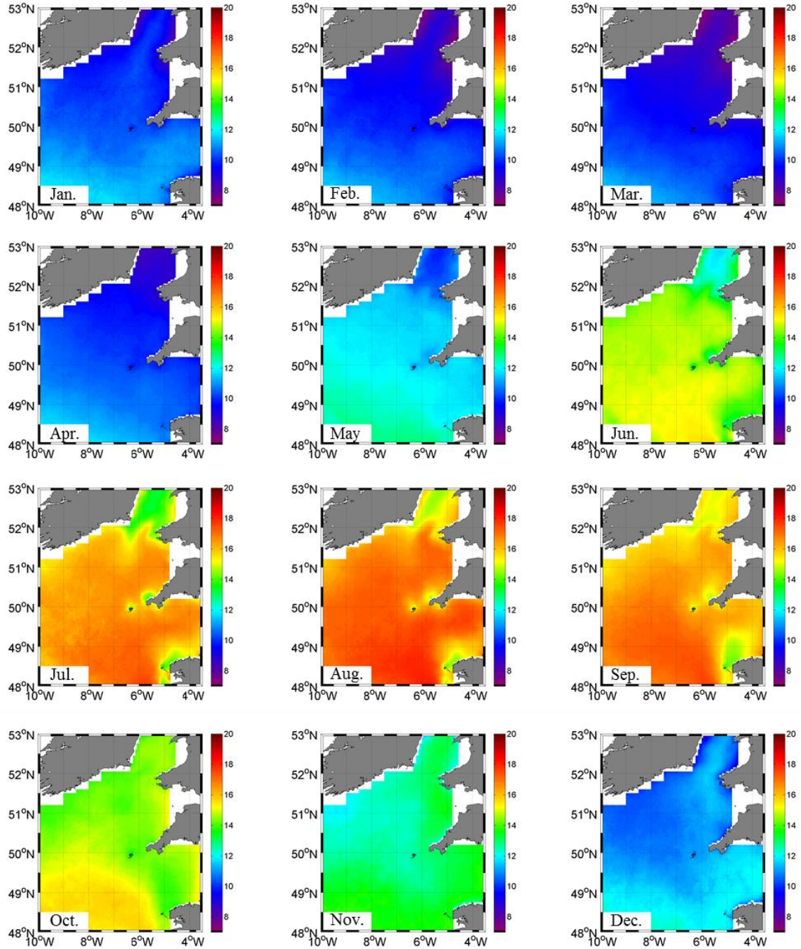
Figure 32: Monthly satellite SST (°C) averaged from 2003 to 2013 from January (top left corner) to December (bottom right corner).
