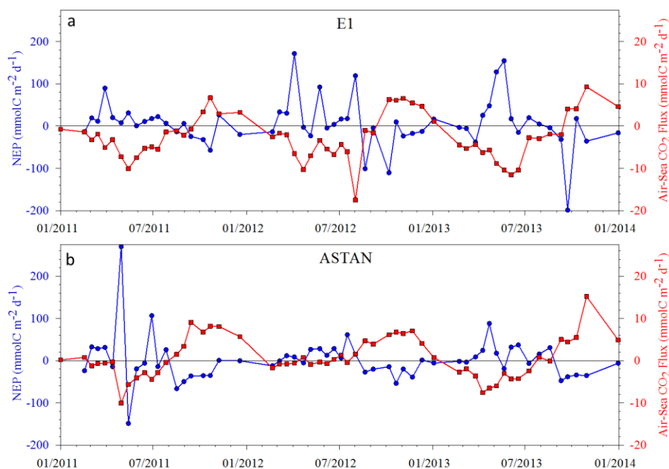
Figure 16: Estimated net ecosystem production (NEP in \text{mmol C m}^{-2} \text{d}^{-1} , blue circles) and air-sea \text{CO}_2 fluxes (in \text{mmol C m}^{-2} \text{d}^{-1} , red squares) computed using the gas transfer velocity parameterization given by Nightingale et al. (2000) in the vicinity of ASTAN ( 48.90^\circ\text{N} - 49.10^\circ\text{N} ) and E1 ( 49.80^\circ\text{N} - 50.00^\circ\text{N} ) from January 2011 to December 2013.
