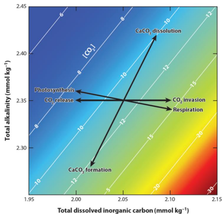
Figure 6: Effect of various processes on the carbonate system parameters (from Zeebe and Wolf-Gladrow, 2001).
