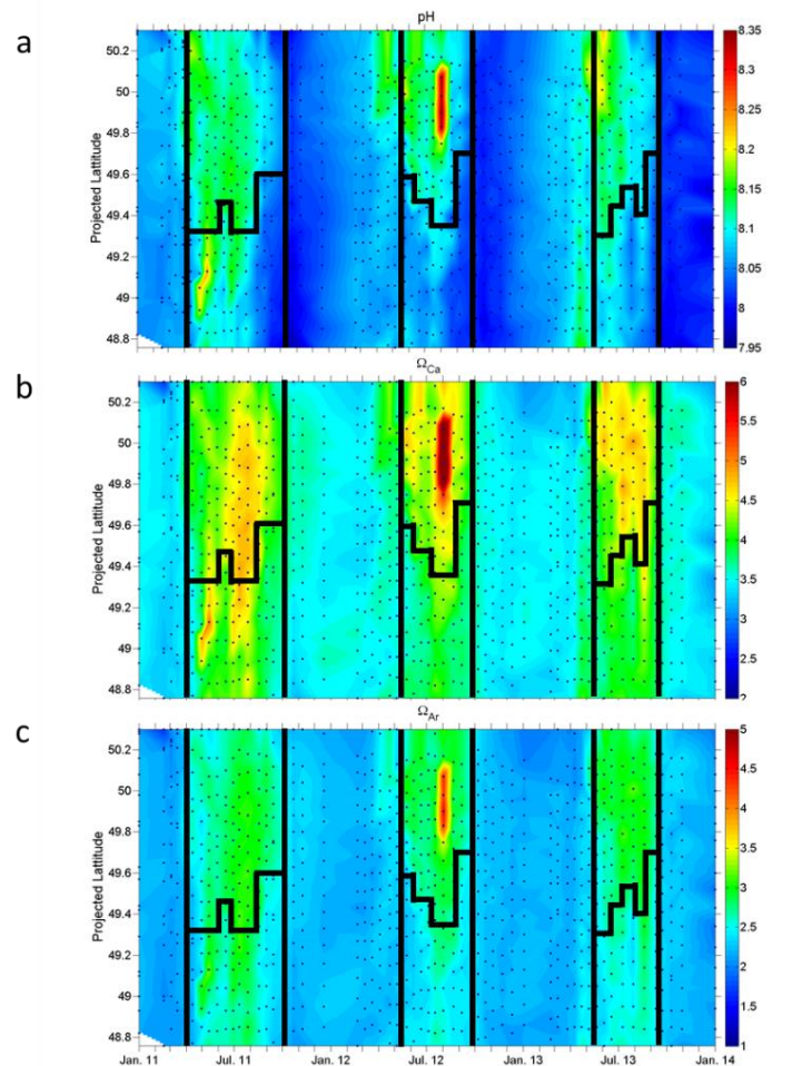
Figure 13: Surface distribution from January 2011 to December 2013 of (A) pH on the total scale, (B) the calcite \Omega_{\text{Ca}} and (C) aragonite \Omega_{\text{Ar}} saturation state in the WEC between Roscoff and Plymouth. Vertical black lines indicate the onset of the breakdown of thermal stratification at fixed station E1 and horizontal black lines represent an estimate of the location of the thermal front (Figure 4).
