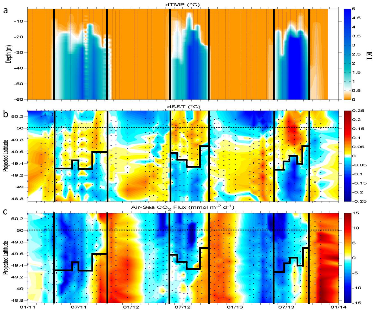
Figure 10: (A) Difference between the surface temperature and the temperatures recorded along the CTD profiles ( dTMP , in ^{\circ}C ) at the fixed station E1 from January 2011 to December 2013. (B) SST anomalies ( dSST , in ^{\circ}C ) from the difference between SST and mean SST for each Roscoff-Plymouth bimonthly transect. (C) Surface distribution from January 2011 to December 2013 of air-sea CO_2 fluxes (in mmol\ C\ m^{-2}\ d^{-1} ) computed with the Nightingale et al. (2000) k-wind parametrization. Vertical black lines indicate the onset of the breakdown of thermal stratification at fixed station E1 and horizontal black lines represent an estimate of the location of the thermal front. The horizontal dotted line indicates the latitudinal location of fixed station E1.
