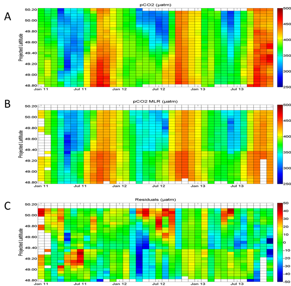
Figure 28: Distribution of monthly gridded (A) p\text{CO}_2 ( \mu\text{atm} ) based on bimonthly DIC/TA measurements (January 2011 to March 2012) and on high-frequency p\text{CO}_2 measurements (April 2012 to December 2013) in WEC, (B) p\text{CO}_{2,\text{MLR}} ( \mu\text{atm} ) computed from nWEC and sWEC algorithms and (C) residuals ( p\text{CO}_{2,\text{obs}} - p\text{CO}_{2,\text{MLR}} in \mu\text{atm} ) between Roscoff and Plymouth from January 2011 to December 2013.
