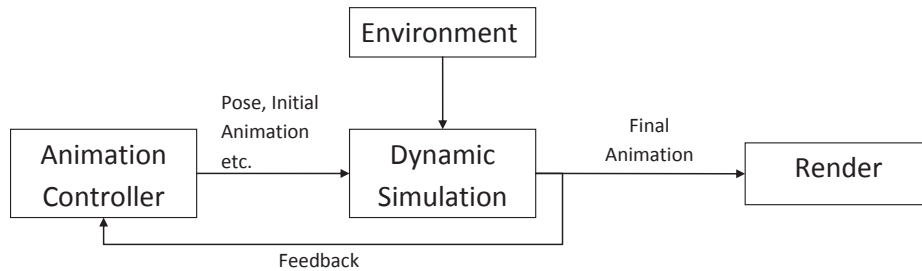
Figure 2.18: Feedback (feed forward) based animation controller.
