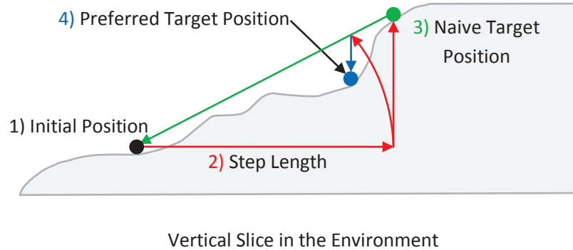
Figure 3.6: How the computation of the preferred footprint target for each foot is done. The vertical slice in the environment can contain objects and obstacles. The naive target position is calculated by querying the environment about the elevation of the 2D point resulted from the initial position + the step length.
