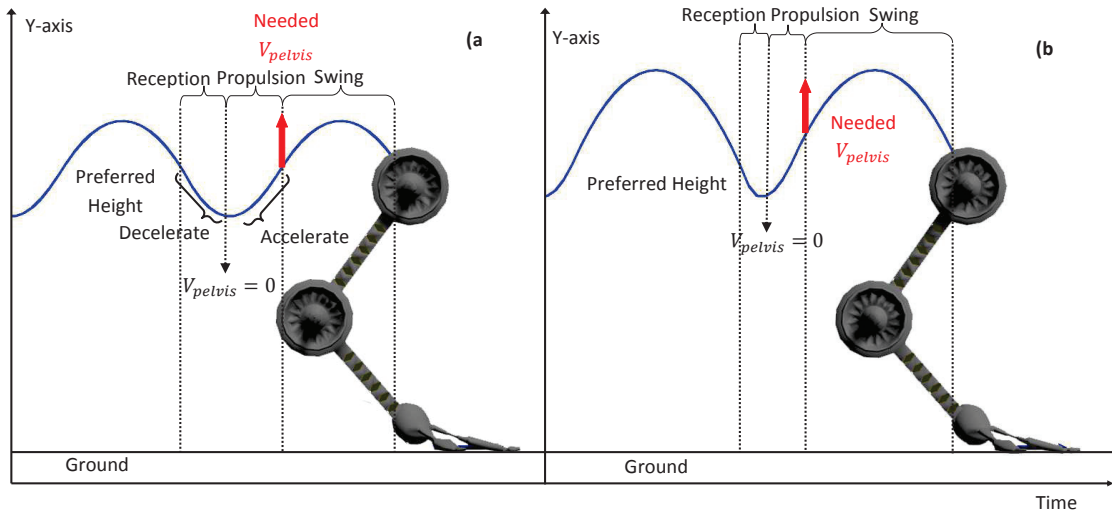
Figure 4.6: Sinusoidal-like ballistic pelvis movement generated implicitly using the foot force calculated based on the reception and propulsion phases. Preferred height is the one fixed by the user. a) Trajectory is generated using the Gait Pattern (a) from Figure 4.5(a). b) Trajectory is generated using the Gait Pattern (b) from Figure 4.5(b).
