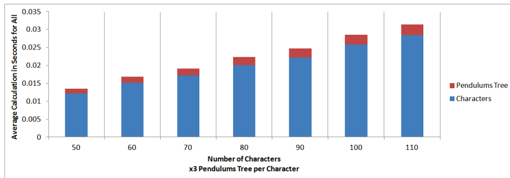
Figure 5.14: Added Calculation time when using pendulums tree in our locomotion system. In seconds.
