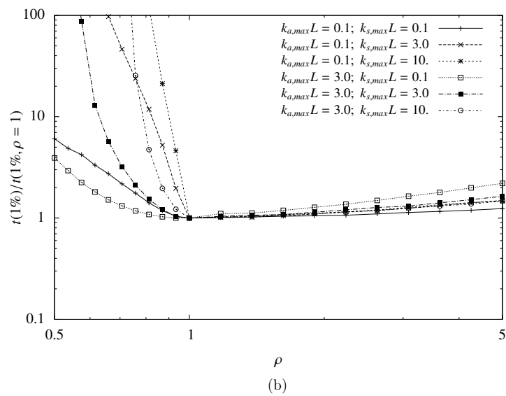
FIGURE D.8 – Computation time in order to reach a 1% standard deviation as a function of \rho , k_{a,max}L , k_{s,max}L at (a) \mathbf{x}_0 = [0, 0, 0] and (b) \mathbf{x}_0 = [-L, 0, 0]
