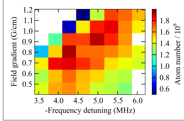
Figure 3.11: 2D optimization data of MOT detuning and magnetic field gradient. Shown is the atom number in the MOT after 10 s loading in color scale as a function of the MOT detuning and the magnetic field gradient in the weak axis of the quadrupole field. Unmeasured points are marked in white.
