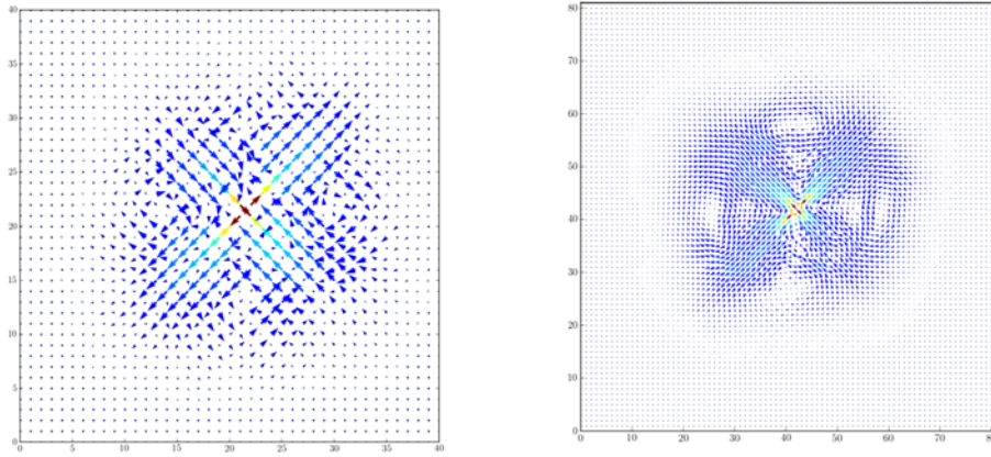
(a) Shear transformation is limited to one element. (b) Shear transformation spans four elements.
