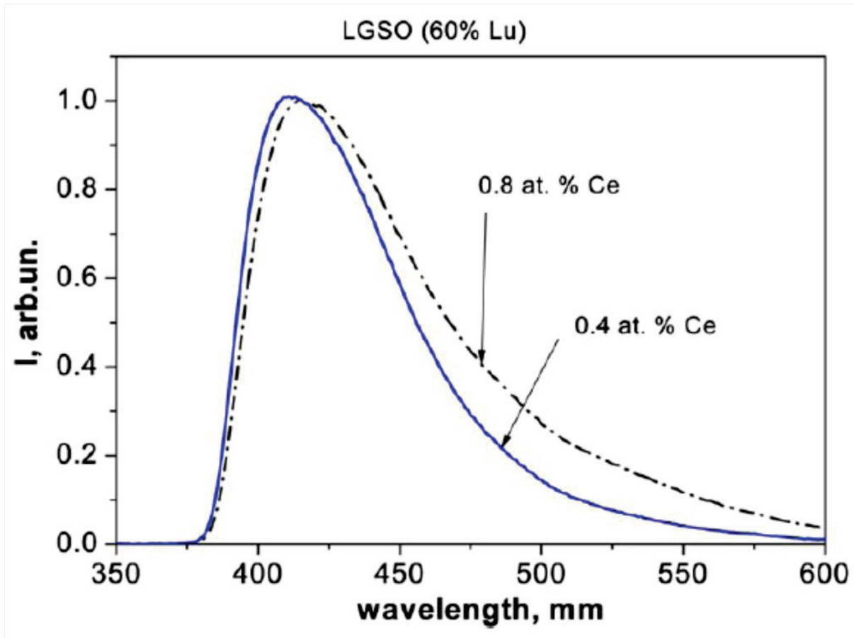
Figure I.17. Red shift of \text{Ce}^{3+} emission on X-ray luminescence spectra for \text{Lu}_{1.2}\text{Gd}_{0.8}\text{SiO}_5:\text{Ce} crystals illustrates the rise of impact from CeO6 centers as common \text{Ce}^{3+} concentration increases [19].
