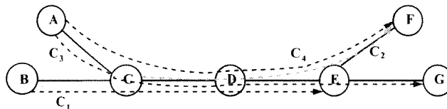
Figure 4.3: Contention Illustration
