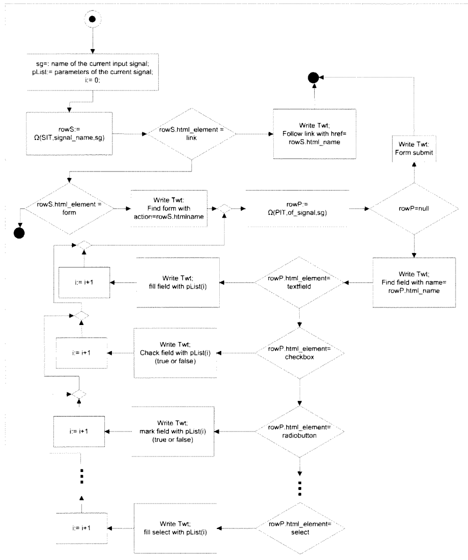
Figure 2.10: Flowchart describing the methodology of the Input instantiation.
