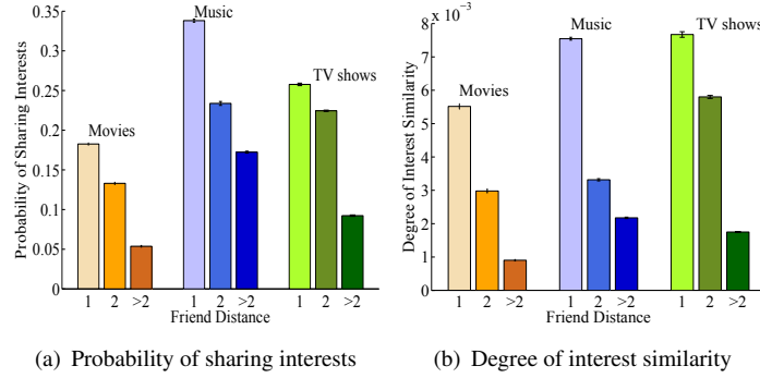
Figure 6.7: Interest similarity by friend distance
