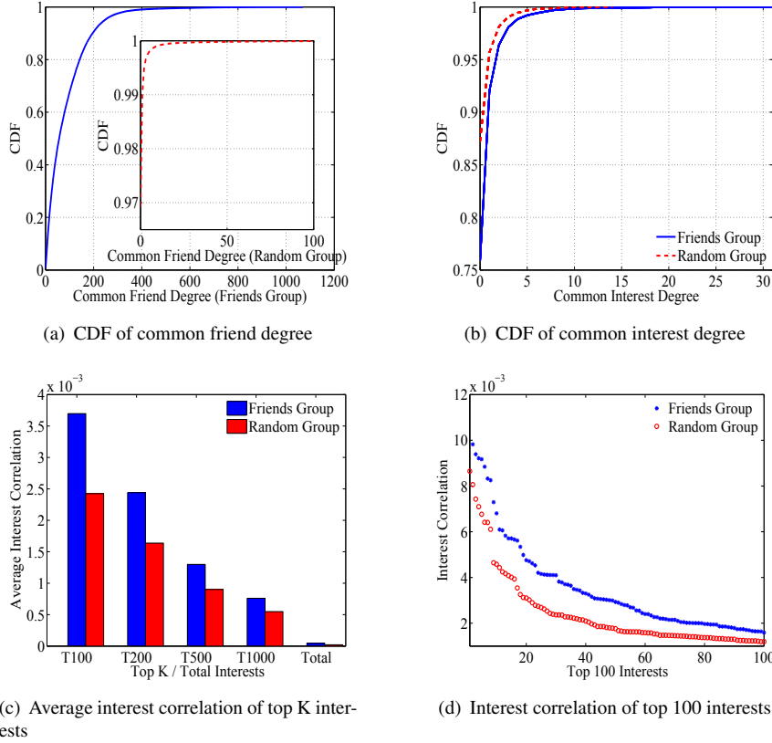
Figure 5.2: User similarity
