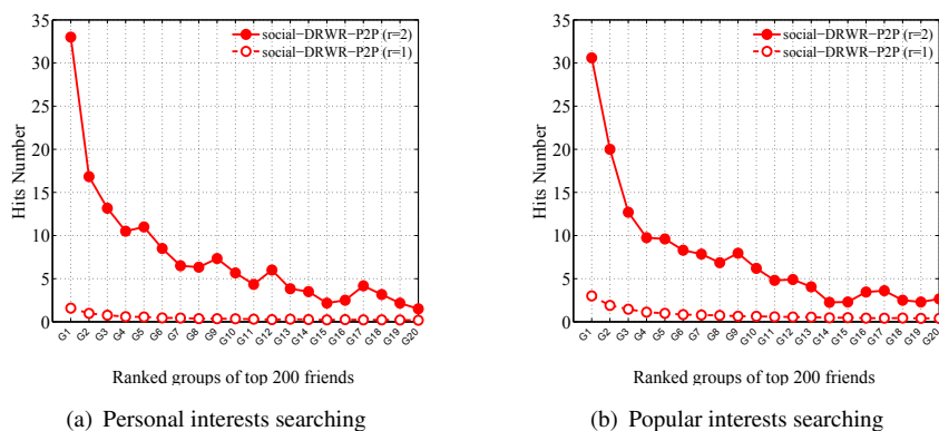
Figure 5.9: Hits number of social-DRWR-P2P
